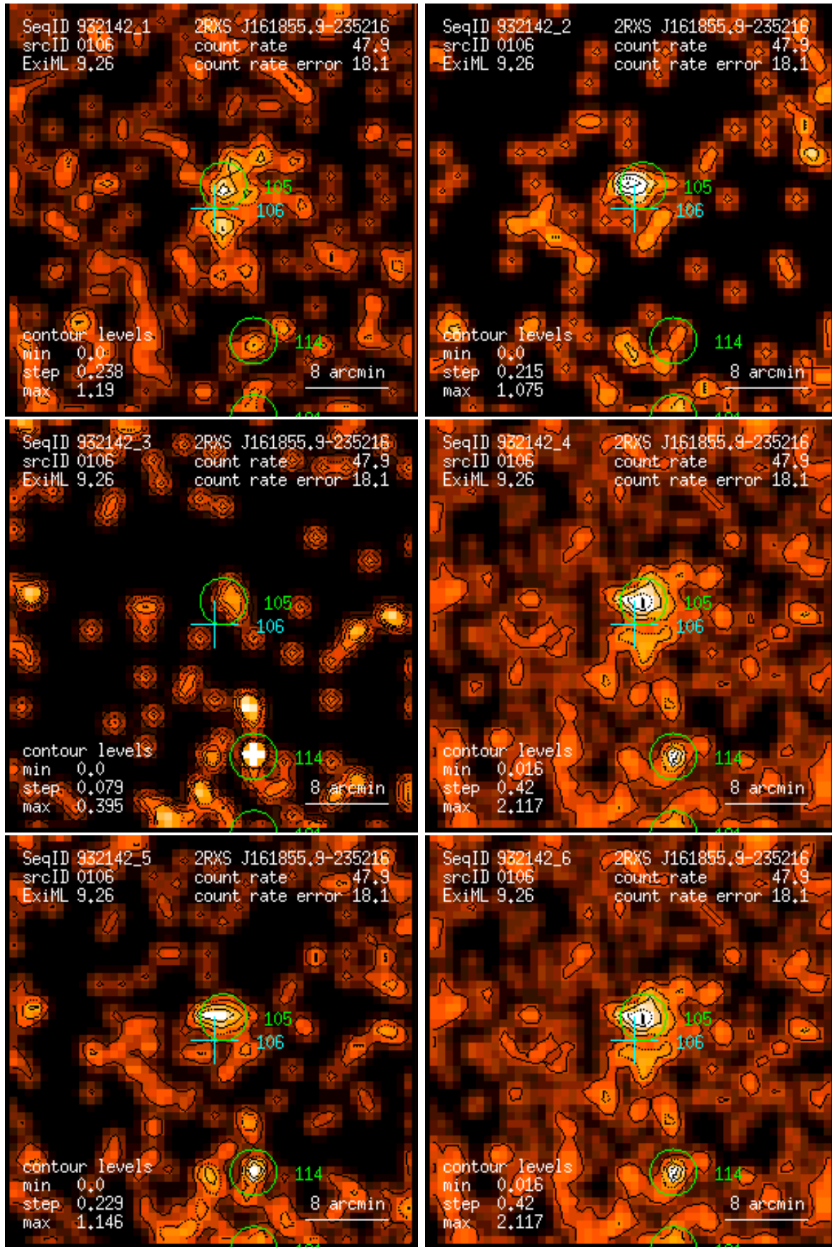
Figure 106: RASS 932142: detection 0106: band rate images, Gaussian filter: (1) PSPC channels 11 – 41, (2) 52 – 90, (3) 91 – 201, (4) 11 – 235, (5) 52 – 201, (6) 11 – 201. Broad band rates in counts/ks. Band rate contour levels in counts/ks/arcmin 2 .
