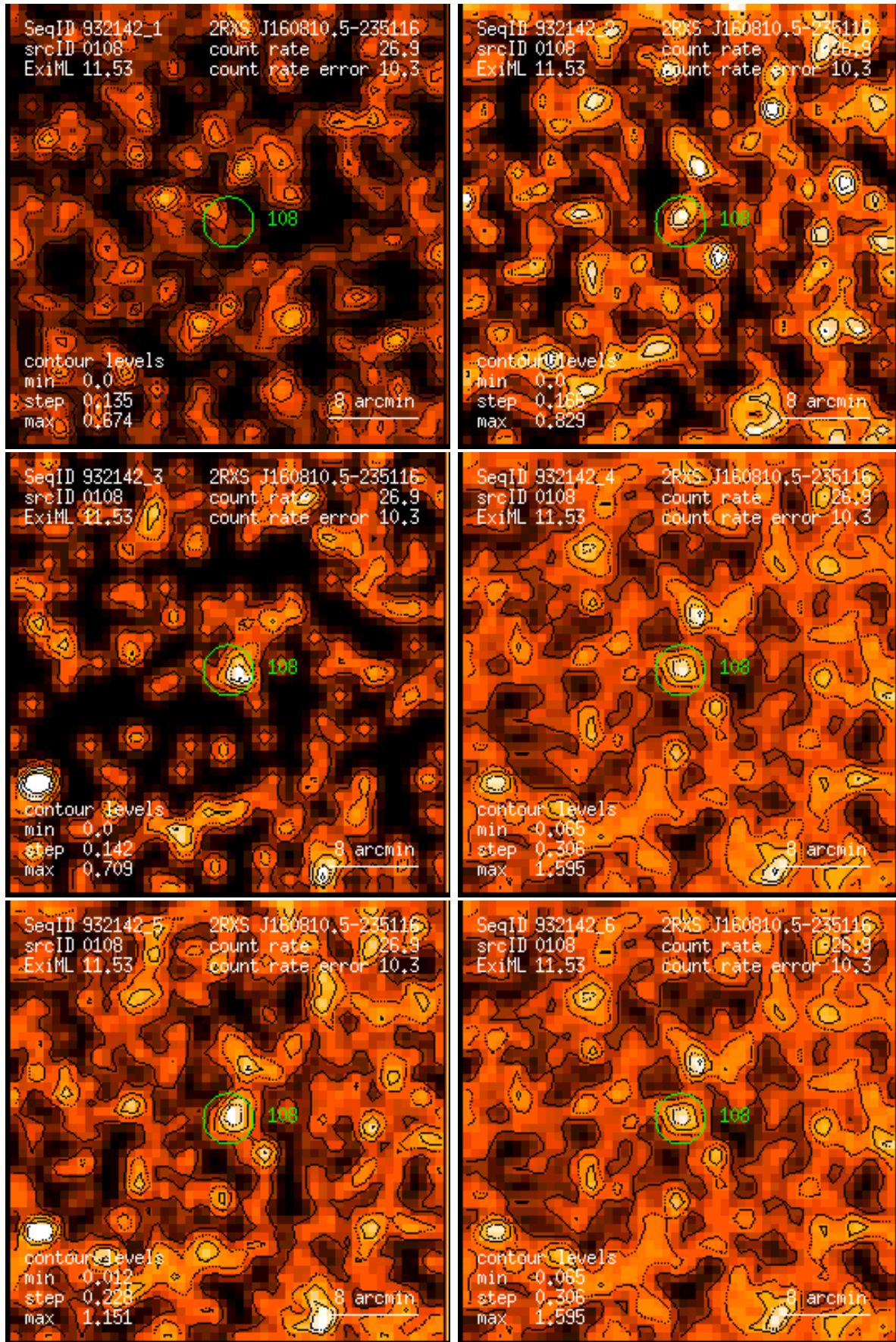
Figure 108: RASS 932142: detection 0108: band rate images, Gaussian filter: (1) PSPC channels 11 – 41, (2) 52 – 90, (3) 91 – 201, (4) 11 – 235, (5) 52 – 201, (6) 11 – 201. Broad band rates in counts/ks. Band rate contour levels in counts/ks/arcmin 2 .
