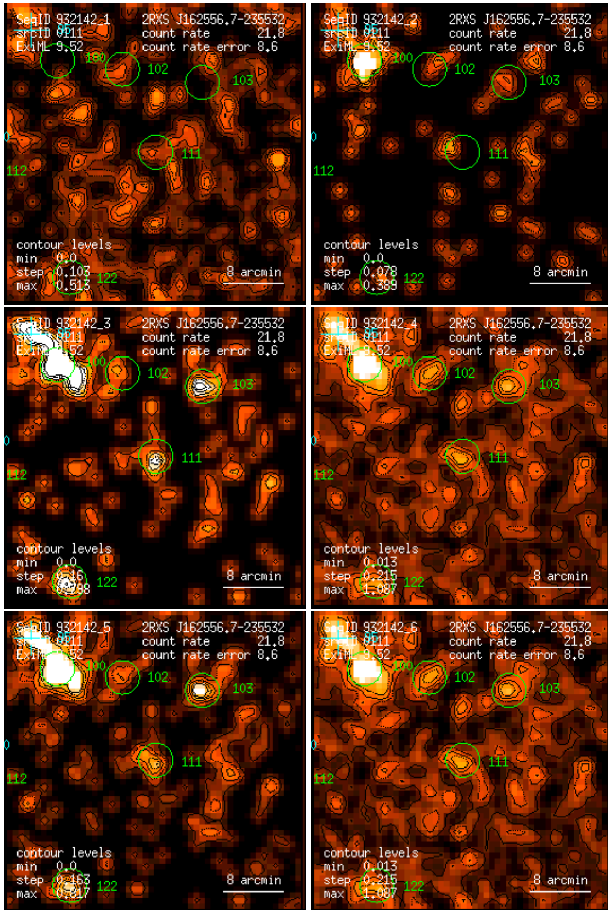
Figure 111: RASS 932142: detection 0111: band rate images, Gaussian filter: (1) PSPC channels 11 – 41, (2) 52 – 90, (3) 91 – 201, (4) 11 – 235, (5) 52 – 201, (6) 11 – 201. Broad band rates in counts/ks. Band rate contour levels in counts/ks/arcmin 2 .
