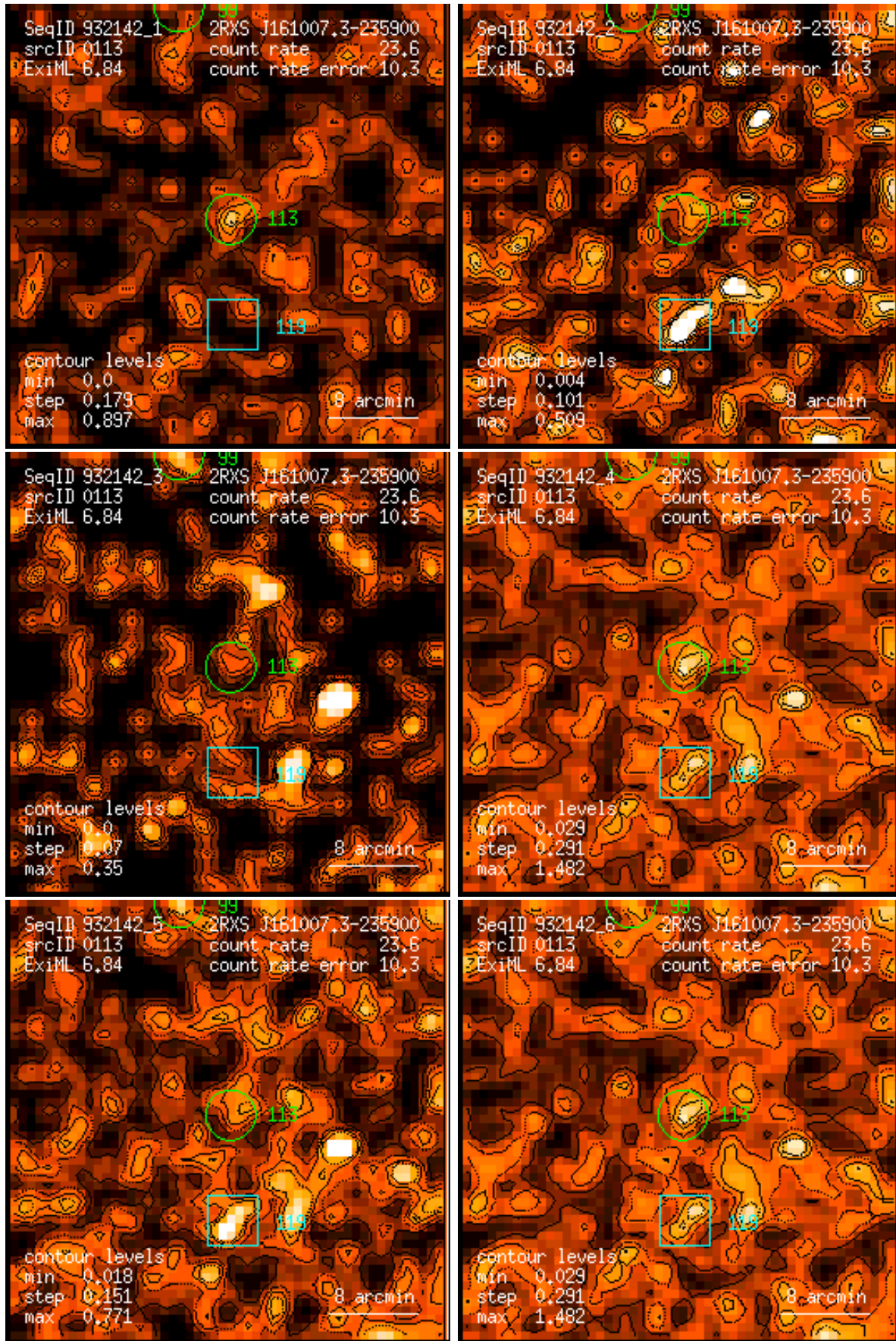
Figure 113: RASS 932142: detection 0113: band rate images, Gaussian filter: (1) PSPC channels 11 – 41, (2) 52 – 90, (3) 91 – 201, (4) 11 – 235, (5) 52 – 201, (6) 11 – 201. Broad band rates in counts/ks. Band rate contour levels in counts/ks/arcmin 2 .
