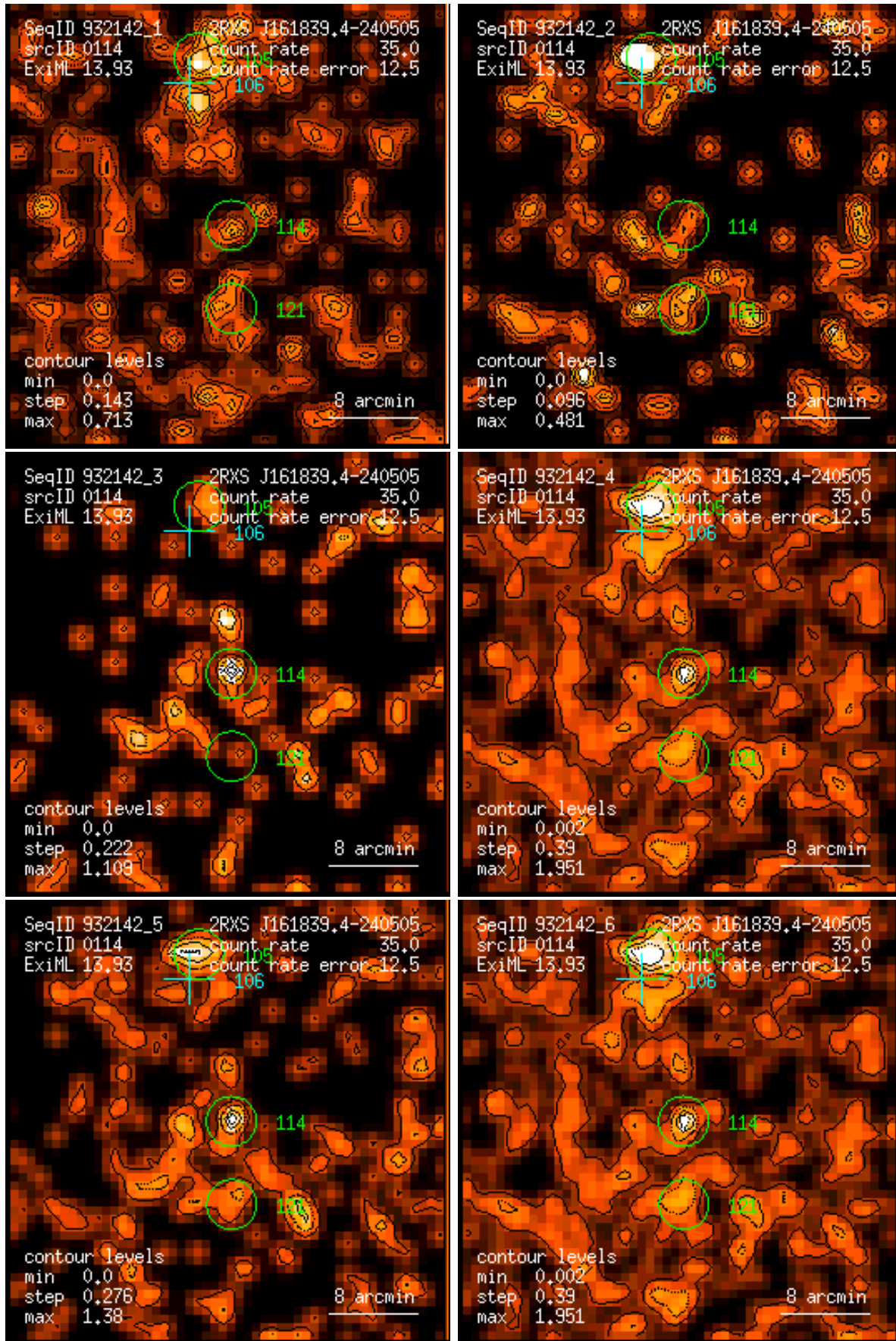
Figure 114: RASS 932142: detection 0114: band rate images, Gaussian filter: (1) PSPC channels 11 – 41, (2) 52 – 90, (3) 91 – 201, (4) 11 – 235, (5) 52 – 201, (6) 11 – 201. Broad band rates in counts/ks. Band rate contour levels in counts/ks/arcmin 2 .
