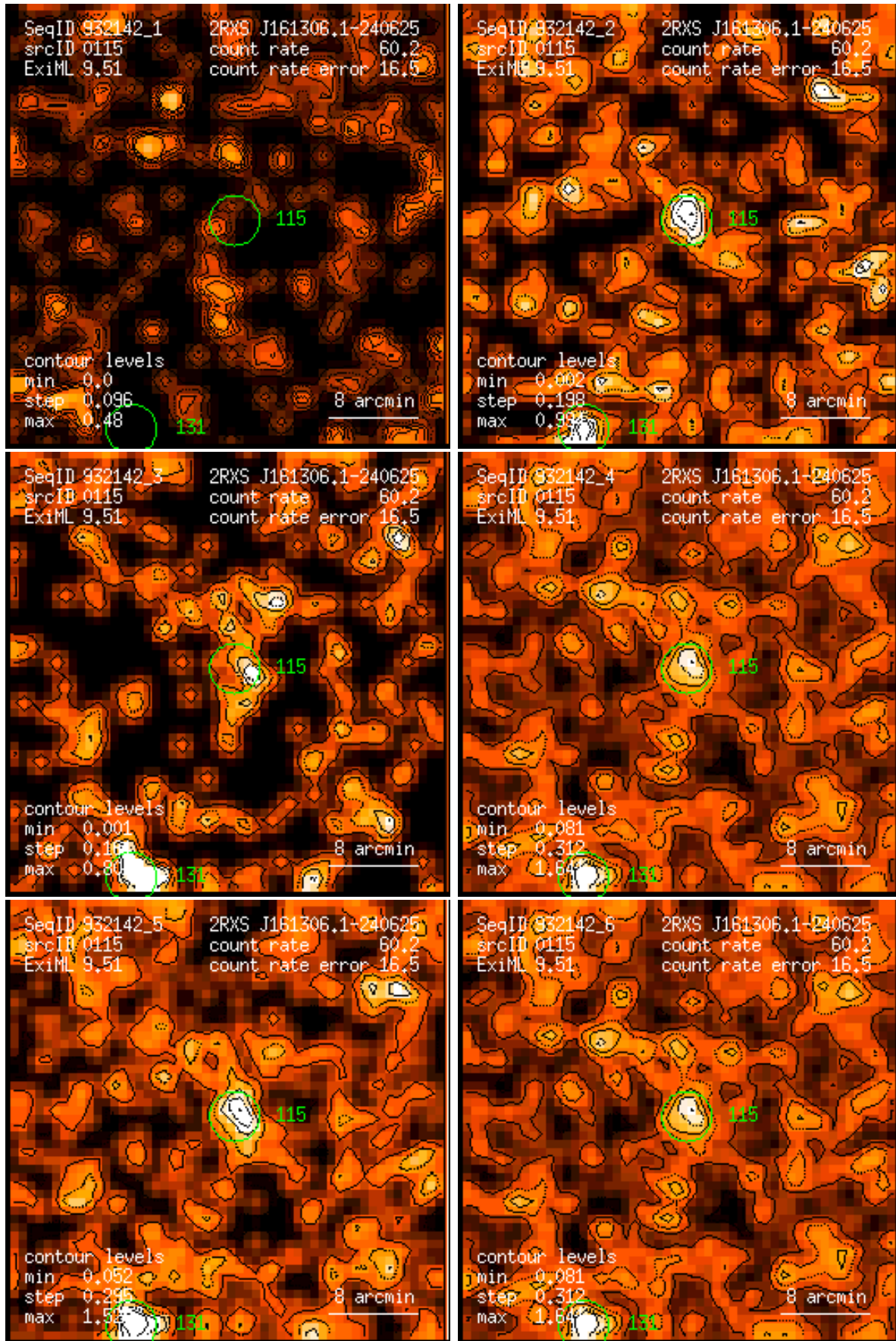
Figure 115: RASS 932142: detection 0115: band rate images, Gaussian filter: (1) PSPC channels 11 – 41, (2) 52 – 90, (3) 91 – 201, (4) 11 – 235, (5) 52 – 201, (6) 11 – 201. Broad band rates in counts/ks. Band rate contour levels in counts/ks/arcmin 2 .
