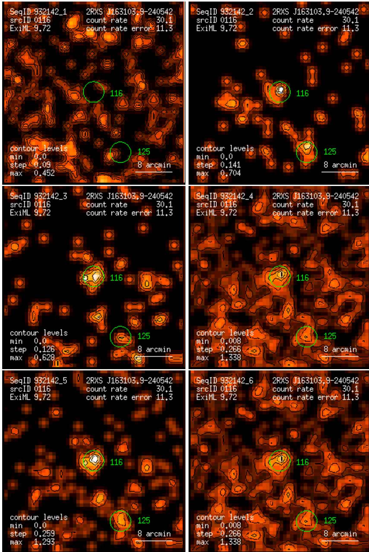
Figure 116: RASS 932142: detection 0116: band rate images, Gaussian filter: (1) PSPC channels 11 – 41, (2) 52 – 90, (3) 91 – 201, (4) 11 – 235, (5) 52 – 201, (6) 11 – 201. Broad band rates in counts/ks. Band rate contour levels in counts/ks/arcmin 2 .
