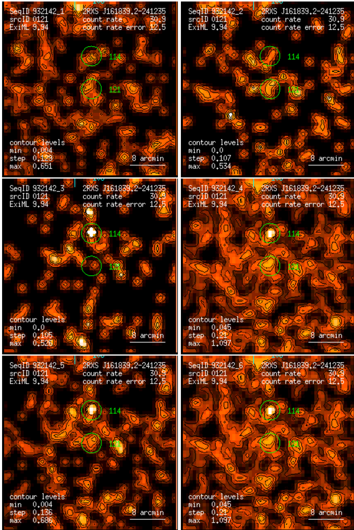
Figure 121: RASS 932142: detection 0121: band rate images, Gaussian filter: (1) PSPC channels 11 – 41, (2) 52 – 90, (3) 91 – 201, (4) 11 – 235, (5) 52 – 201, (6) 11 – 201. Broad band rates in counts/ks. Band rate contour levels in counts/ks/arcmin 2 .
