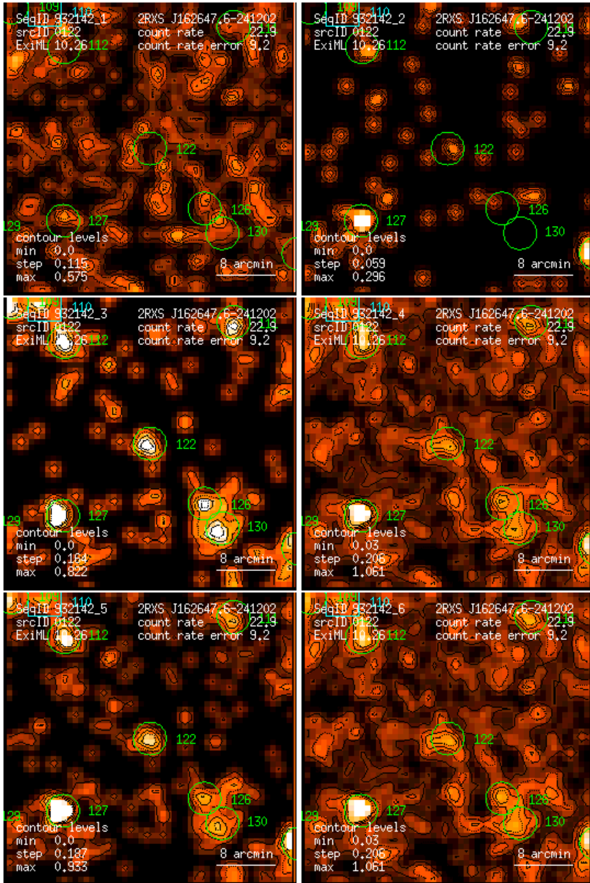
Figure 122: RASS 932142: detection 0122: band rate images, Gaussian filter: (1) PSPC channels 11 – 41, (2) 52 – 90, (3) 91 – 201, (4) 11 – 235, (5) 52 – 201, (6) 11 – 201. Broad band rates in counts/ks. Band rate contour levels in counts/ks/arcmin 2 .
