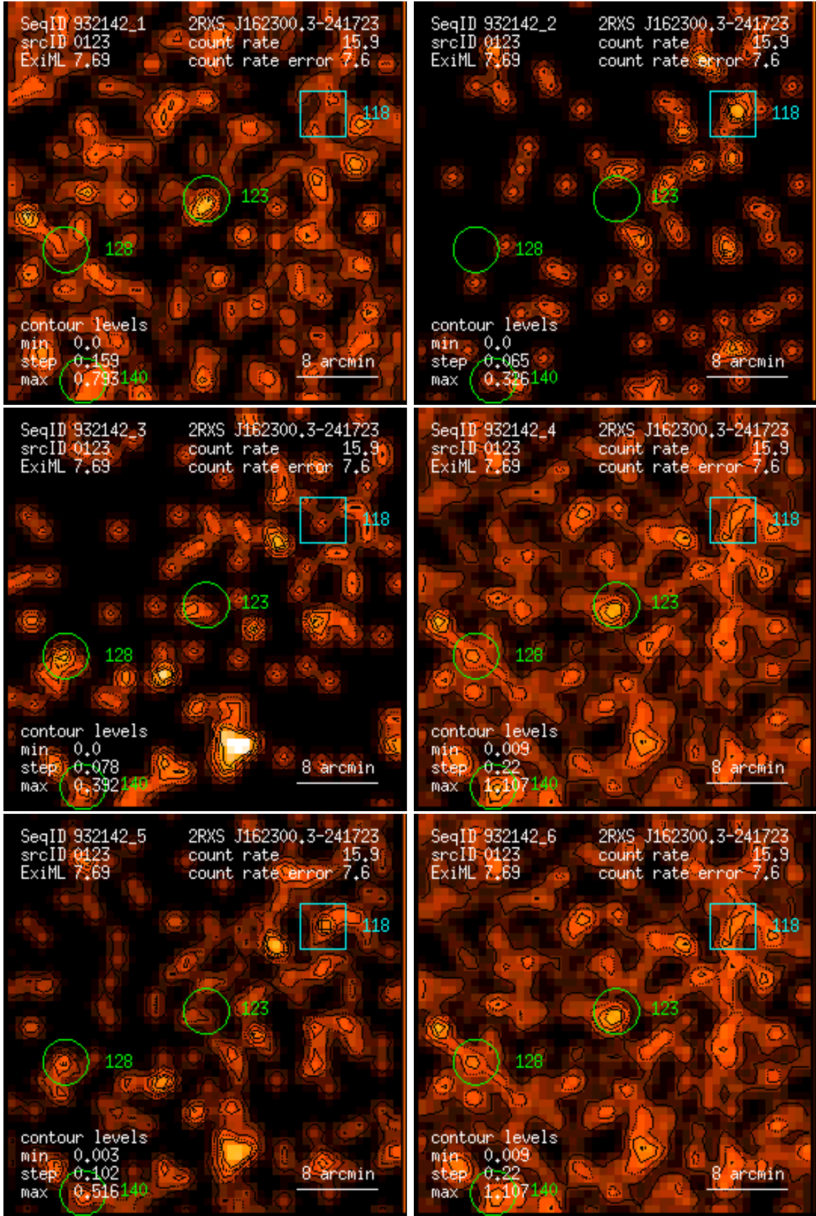
Figure 123: RASS 932142: detection 0123: band rate images, Gaussian filter: (1) PSPC channels 11 – 41, (2) 52 – 90, (3) 91 – 201, (4) 11 – 235, (5) 52 – 201, (6) 11 – 201. Broad band rates in counts/ks. Band rate contour levels in counts/ks/arcmin 2 .
