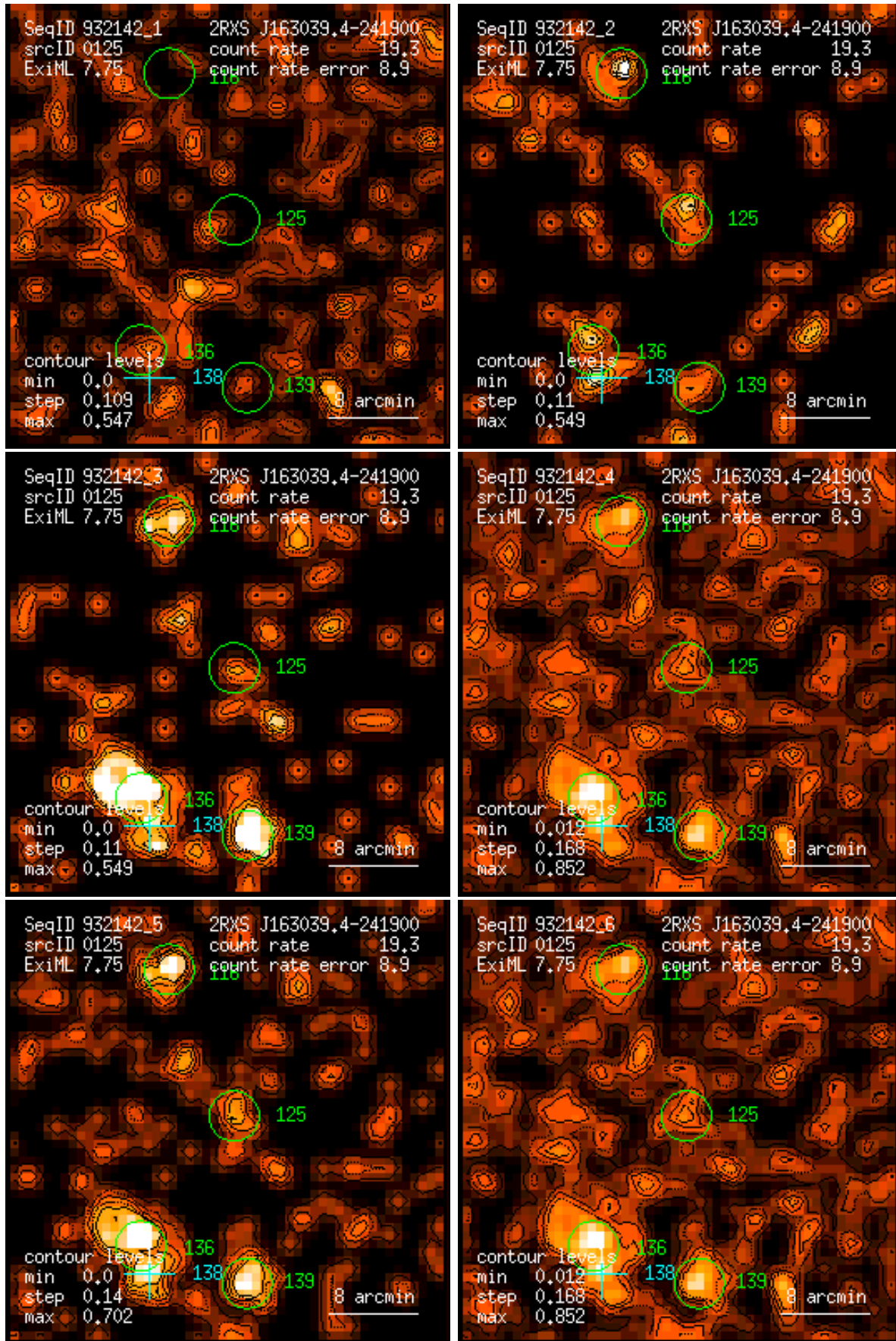
Figure 125: RASS 932142: detection 0125: band rate images, Gaussian filter: (1) PSPC channels 11 – 41, (2) 52 – 90, (3) 91 – 201, (4) 11 – 235, (5) 52 – 201, (6) 11 – 201. Broad band rates in counts/ks. Band rate contour levels in counts/ks/arcmin 2 .
