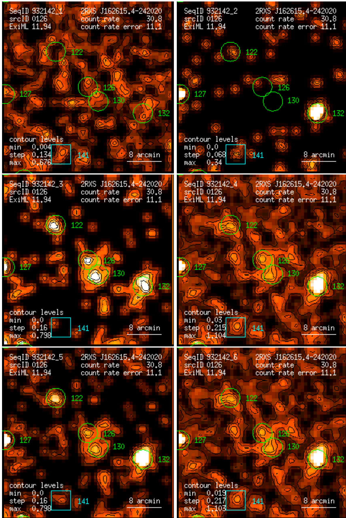
Figure 126: RASS 932142: detection 0126: band rate images, Gaussian filter: (1) PSPC channels 11 – 41, (2) 52 – 90, (3) 91 – 201, (4) 11 – 235, (5) 52 – 201, (6) 11 – 201. Broad band rates in counts/ks. Band rate contour levels in counts/ks/arcmin 2 .
