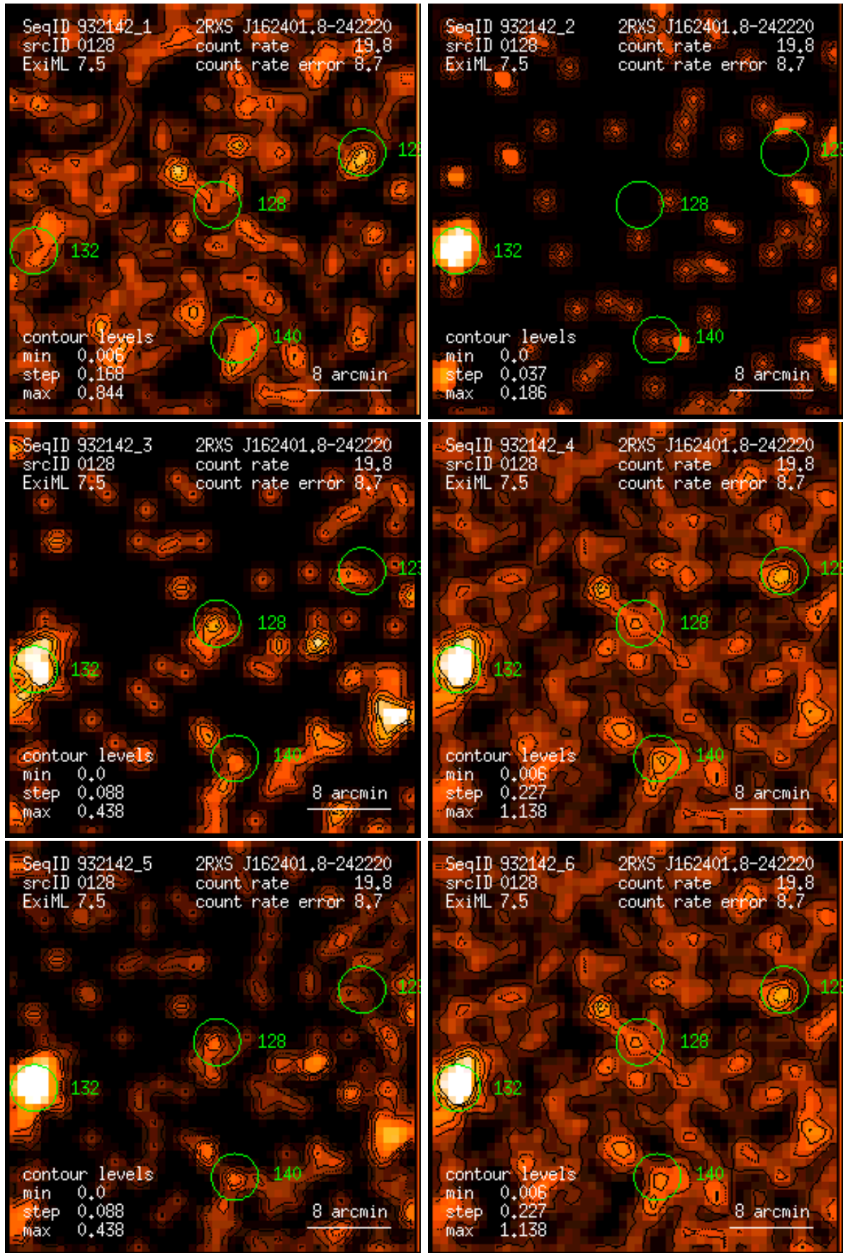
Figure 128: RASS 932142: detection 0128: band rate images, Gaussian filter: (1) PSPC channels 11 – 41, (2) 52 – 90, (3) 91 – 201, (4) 11 – 235, (5) 52 – 201, (6) 11 – 201. Broad band rates in counts/ks. Band rate contour levels in counts/ks/arcmin 2 .
