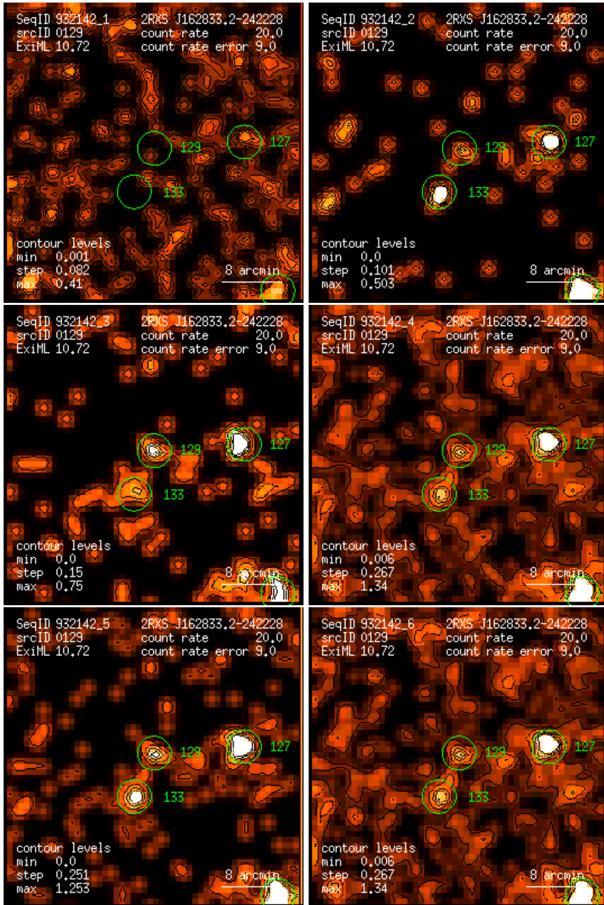
Figure 129: RASS 932142: detection 0129: band rate images, Gaussian filter: (1) PSPPC channels 11 – 41, (2) 52 – 90, (3) 91 – 201, (4) 11 – 235, (5) 52 – 201, (6) 11 – 201. Broad band rates in counts/ks. Band rate contour levels in counts/ks/arcmin 2 .
