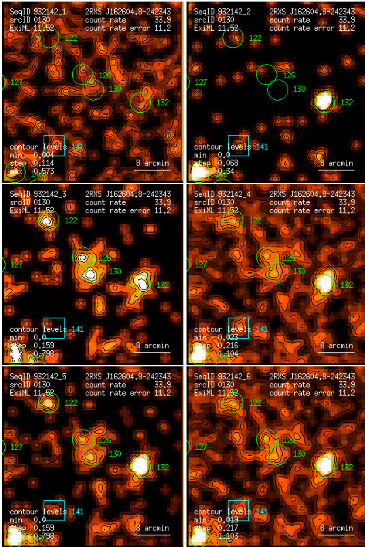
Figure 130: RASS 932142: detection 0130: band rate images, Gaussian filter: (1) PSPC channels 11 – 41, (2) 52 – 90, (3) 91 – 201, (4) 11 – 235, (5) 52 – 201, (6) 11 – 201. Broad band rates in counts/ks. Band rate contour levels in counts/ks/arcmin 2 .
