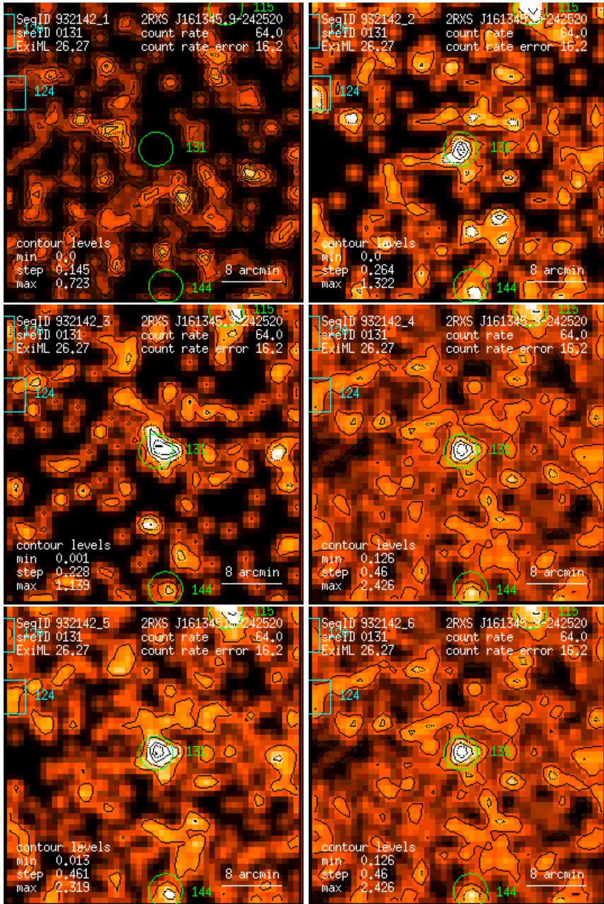
Figure 131: RASS 932142: detection 0131: band rate images, Gaussian filter: (1) PSPC channels 11 – 41, (2) 52 – 90, (3) 91 – 201, (4) 11 – 235, (5) 52 – 201, (6) 11 – 201. Broad band rates in counts/ks. Band rate contour levels in counts/ks/arcmin 2 .
