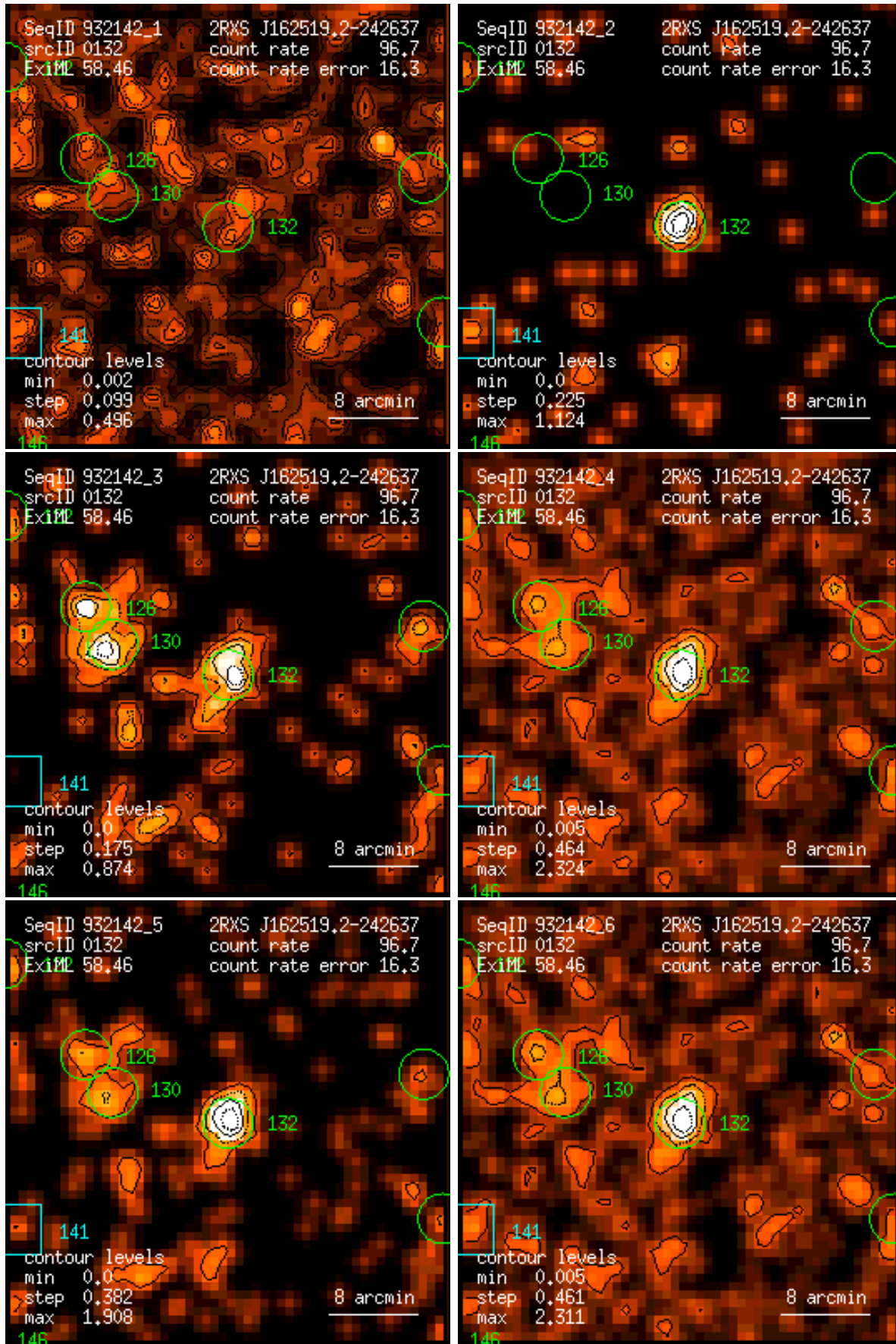
Figure 132: RASS 932142: detection 0132: band rate images, Gaussian filter: (1) PSPC channels 11 – 41, (2) 52 – 90, (3) 91 – 201, (4) 11 – 235, (5) 52 – 201, (6) 11 – 201. Broad band rates in counts/ks. Band rate contour levels in counts/ks/arcmin 2 .
