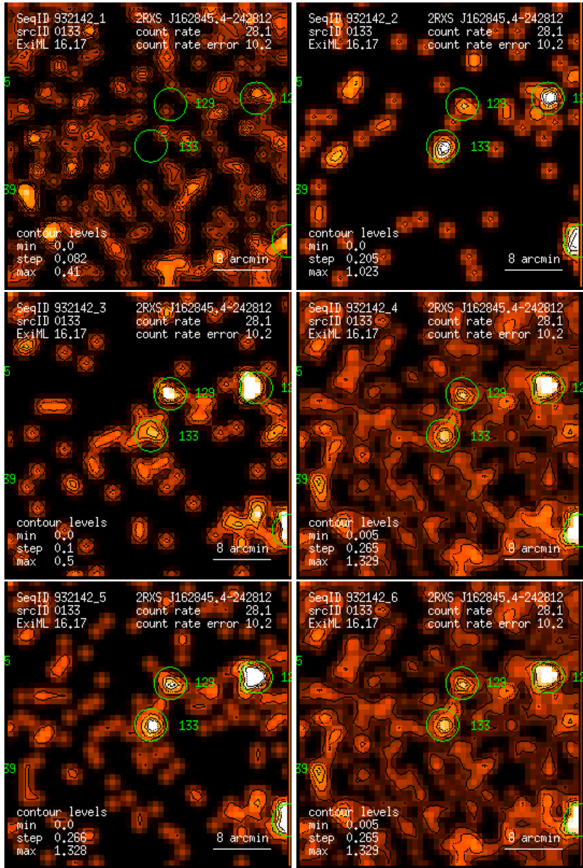
Figure 133: RASS 932142: detection 0133: band rate images, Gaussian filter: (1) PSPC channels 11 – 41, (2) 52 – 90, (3) 91 – 201, (4) 11 – 235, (5) 52 – 201, (6) 11 – 201. Broad band rates in counts/ks. Band rate contour levels in counts/ks/arcmin 2 .
