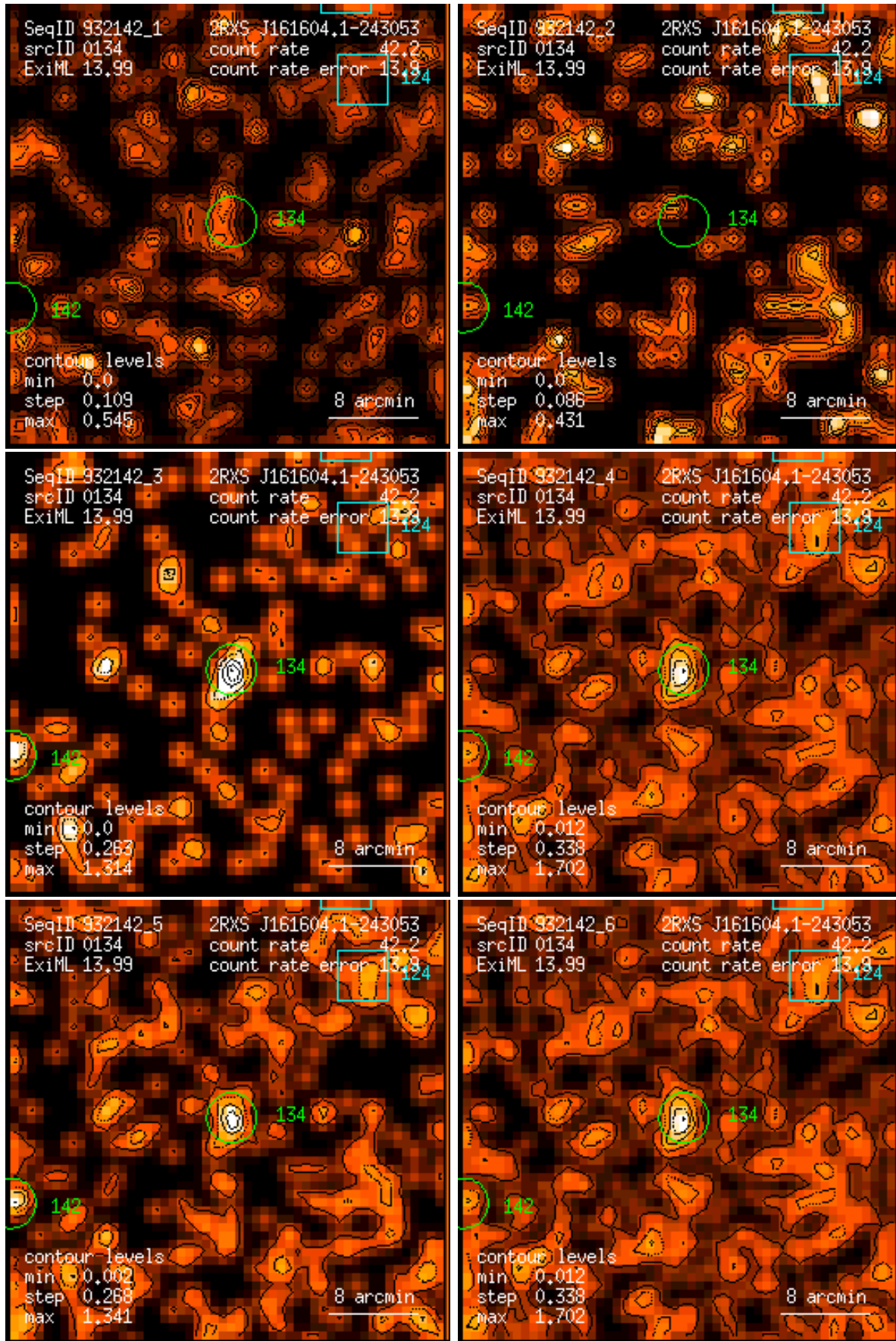
Figure 134: RASS 932142: detection 0134: band rate images, Gaussian filter: (1) PSPC channels 11 – 41, (2) 52 – 90, (3) 91 – 201, (4) 11 – 235, (5) 52 – 201, (6) 11 – 201. Broad band rates in counts/ks. Band rate contour levels in counts/ks/arcmin 2 .
