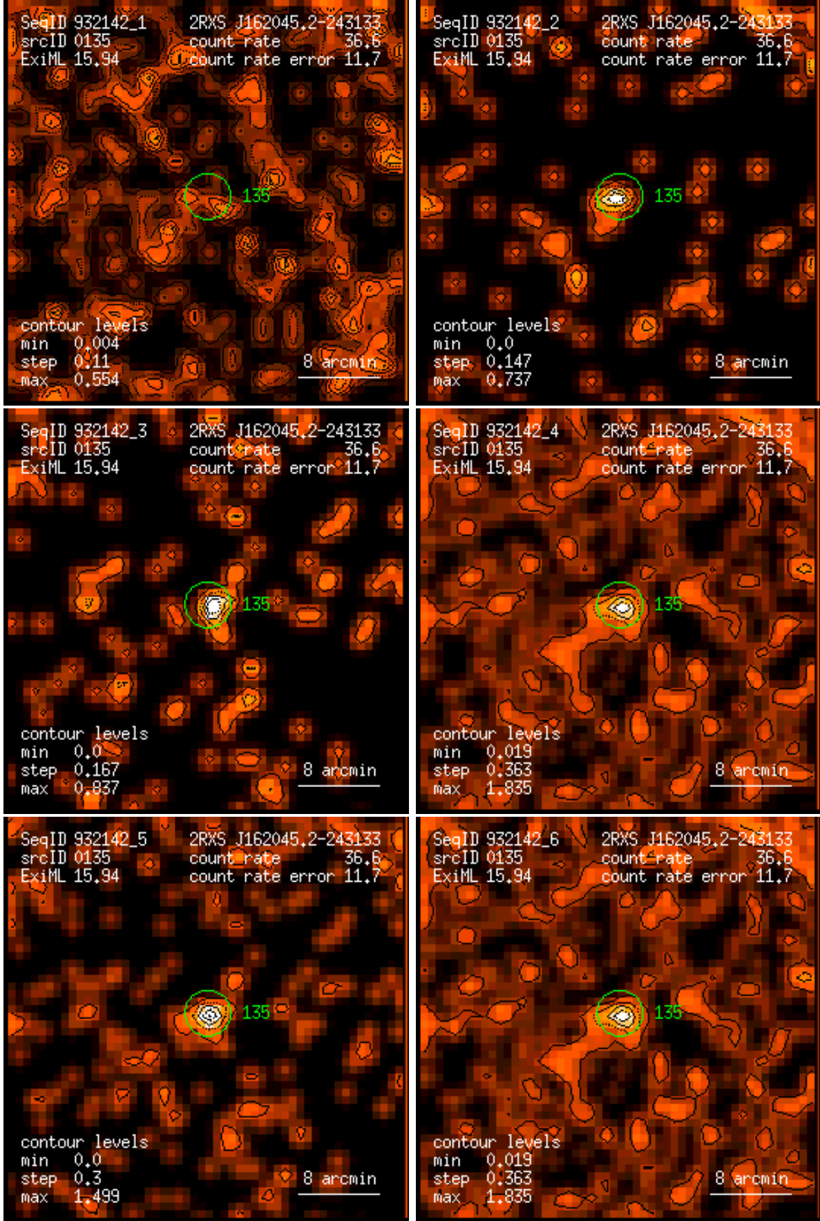
Figure 135: RASS 932142: detection 0135: band rate images, Gaussian filter: (1) PSPC channels 11 – 41, (2) 52 – 90, (3) 91 – 201, (4) 11 – 235, (5) 52 – 201, (6) 11 – 201. Broad band rates in counts/ks. Band rate contour levels in counts/ks/arcmin 2 .
