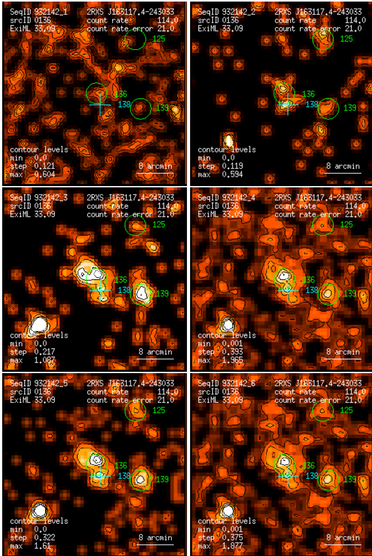
Figure 136: RASS 932142: detection 0136: band rate images, Gaussian filter: (1) PSPC channels 11 – 41, (2) 52 – 90, (3) 91 – 201, (4) 11 – 235, (5) 52 – 201, (6) 11 – 201. Broad band rates in counts/ks. Band rate contour levels in counts/ks/arcmin 2 .
