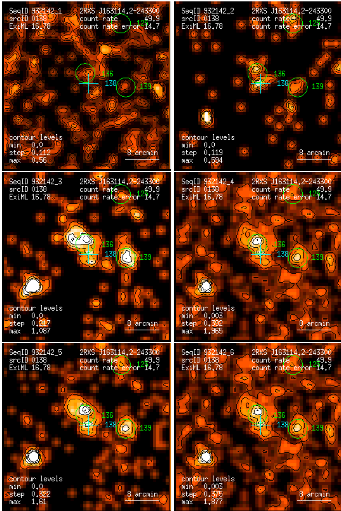
Figure 138: RASS 932142: detection 0138: band rate images, Gaussian filter: (1) PSPC channels 11 – 41, (2) 52 – 90, (3) 91 – 201, (4) 11 – 235, (5) 52 – 201, (6) 11 – 201. Broad band rates in counts/ks. Band rate contour levels in counts/ks/arcmin 2 .
