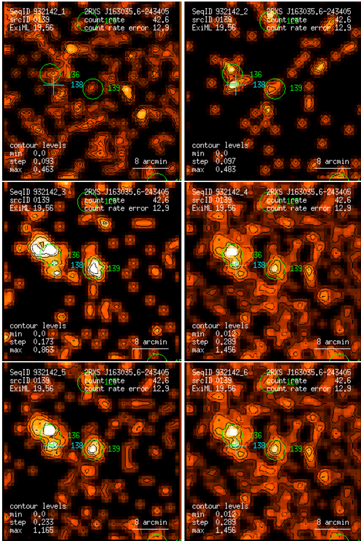
Figure 139: RASS 932142: detection 0139: band rate images, Gaussian filter: (1) PSPC channels 11 – 41, (2) 52 – 90, (3) 91 – 201, (4) 11 – 235, (5) 52 – 201, (6) 11 – 201. Broad band rates in counts/ks. Band rate contour levels in counts/ks/arcmin 2 .
