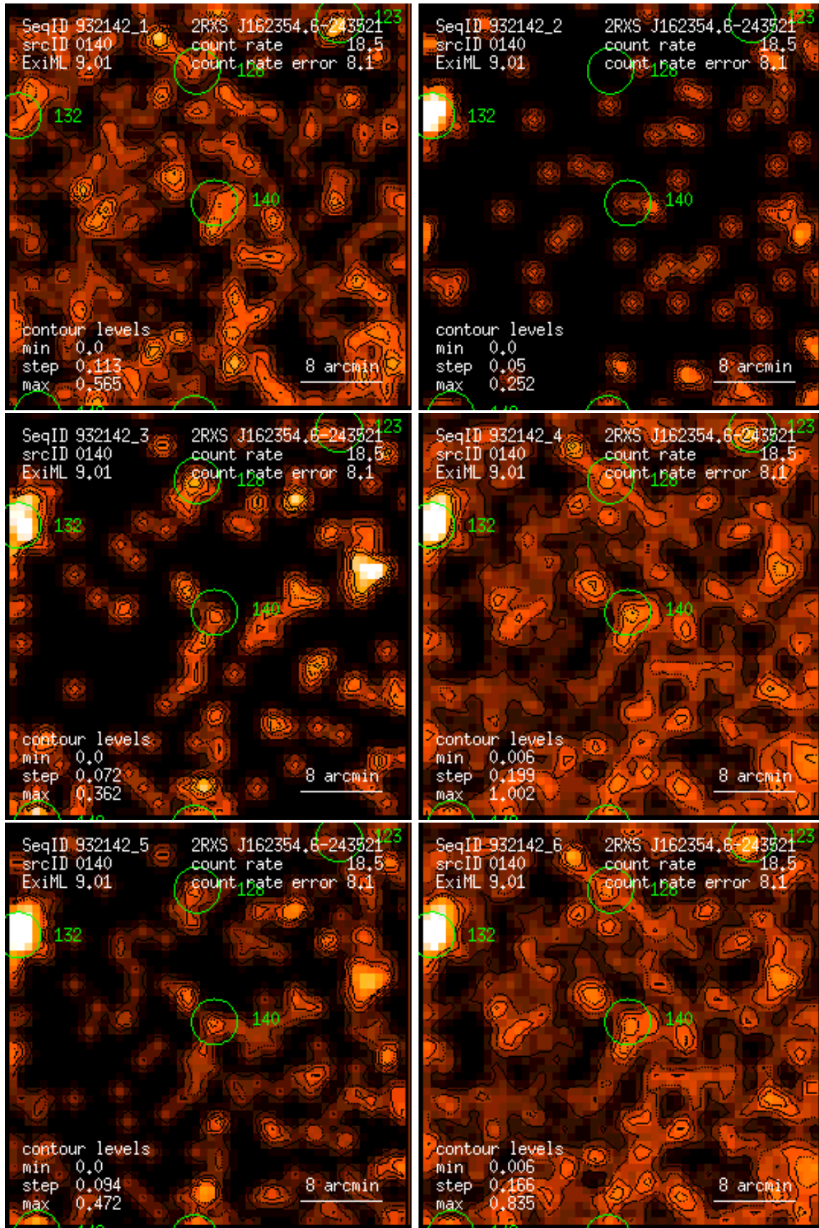
Figure 140: RASS 932142: detection 0140: band rate images, Gaussian filter: (1) PSPC channels 11 – 41, (2) 52 – 90, (3) 91 – 201, (4) 11 – 235, (5) 52 – 201, (6) 11 – 201. Broad band rates in counts/ks. Band rate contour levels in counts/ks/arcmin 2 .
