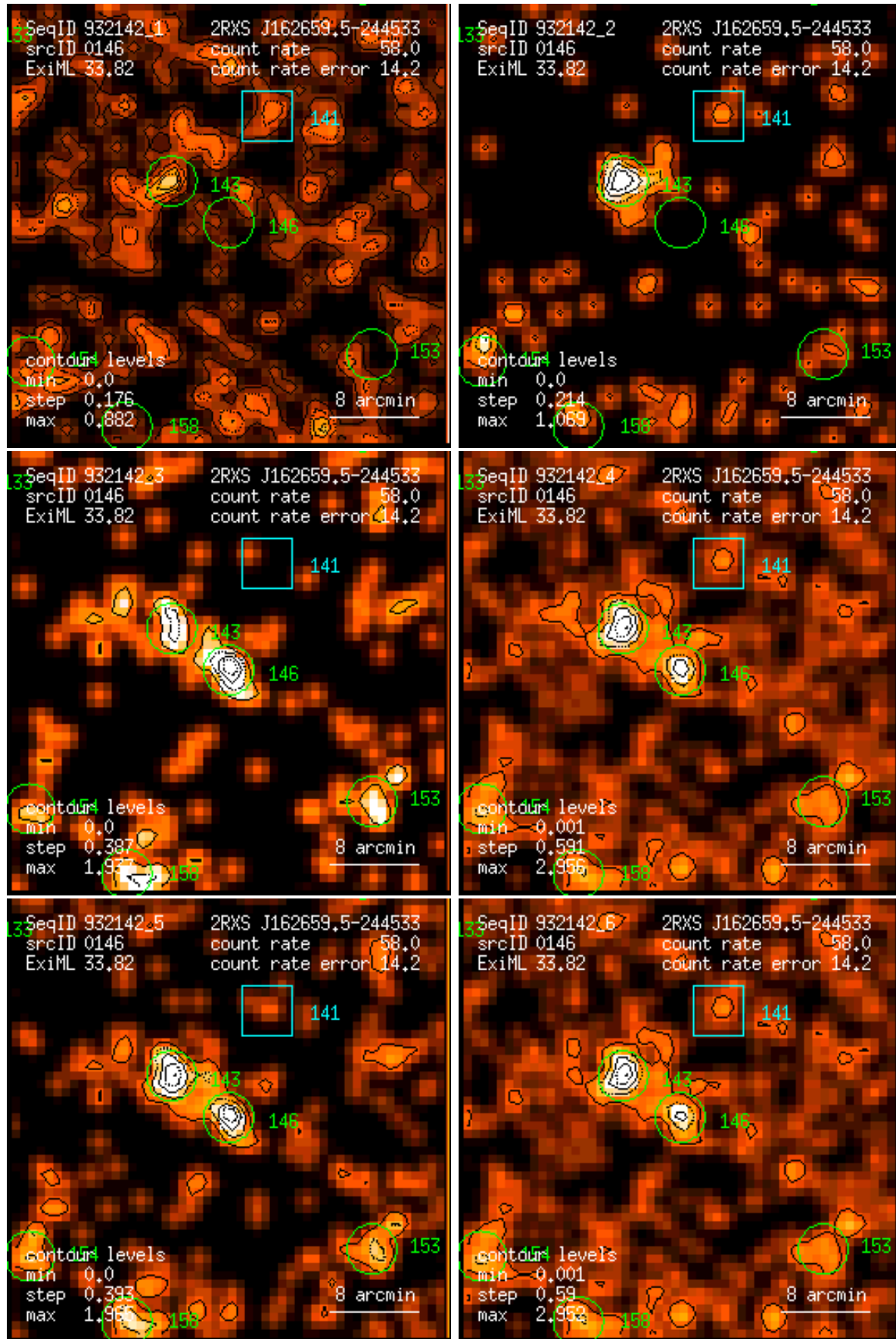
Figure 146: RASS 932142: detection 0146: band rate images, Gaussian filter: (1) PSPC channels 11 – 41, (2) 52 – 90, (3) 91 – 201, (4) 11 – 235, (5) 52 – 201, (6) 11 – 201. Broad band rates in counts/ks. Band rate contour levels in counts/ks/arcmin 2 .
