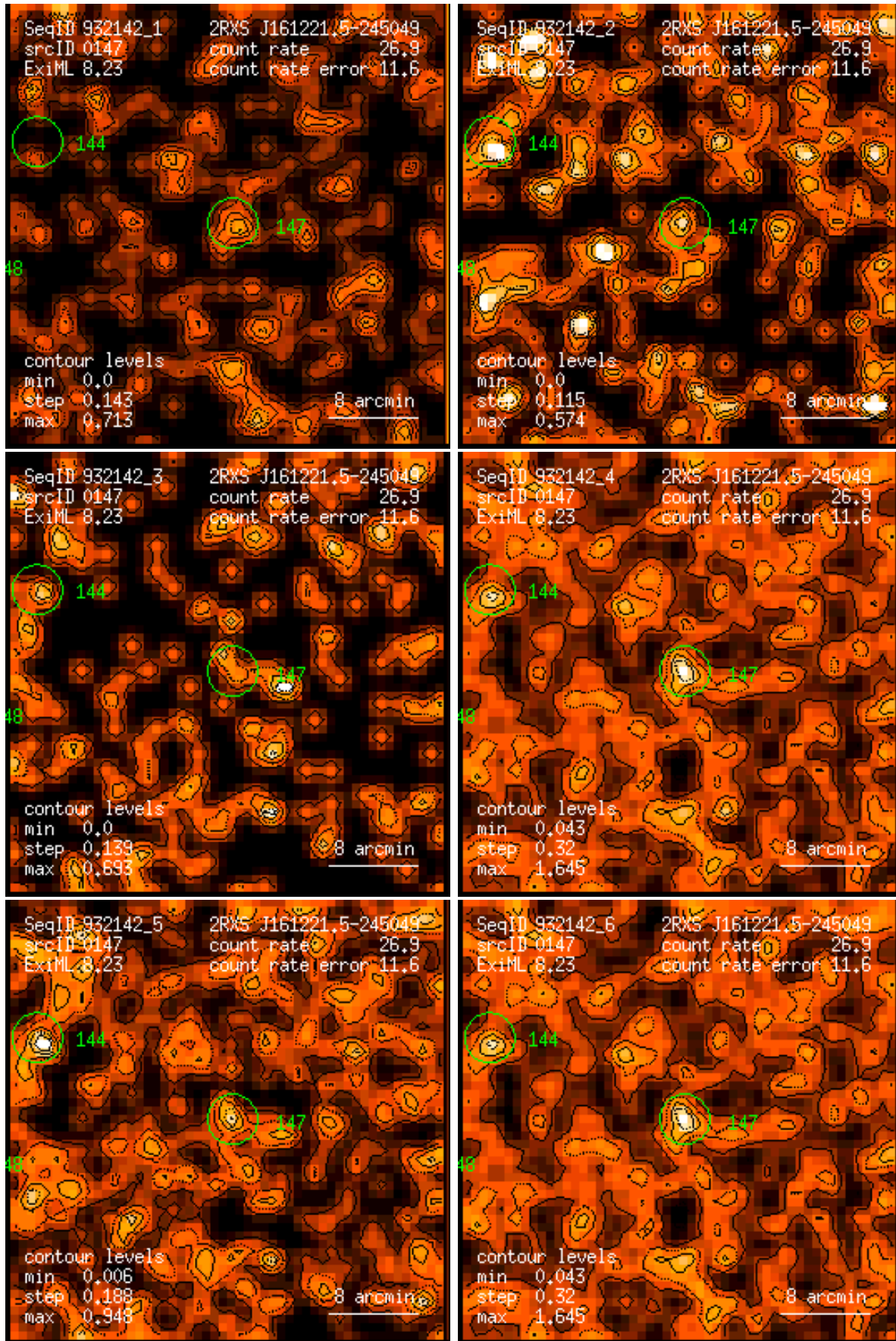
Figure 147: RASS 932142: detection 0147: band rate images, Gaussian filter: (1) PSPC channels 11 – 41, (2) 52 – 90, (3) 91 – 201, (4) 11 – 235, (5) 52 – 201, (6) 11 – 201. Broad band rates in counts/ks. Band rate contour levels in counts/ks/arcmin 2 .
