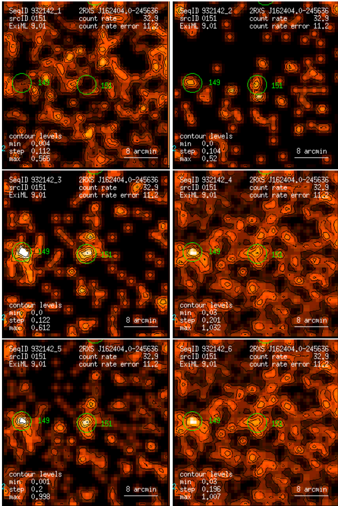
Figure 151: RASS 932142: detection 0151: band rate images, Gaussian filter: (1) PSPC channels 11 – 41, (2) 52 – 90, (3) 91 – 201, (4) 11 – 235, (5) 52 – 201, (6) 11 – 201. Broad band rates in counts/ks. Band rate contour levels in counts/ks/arcmin 2 .
