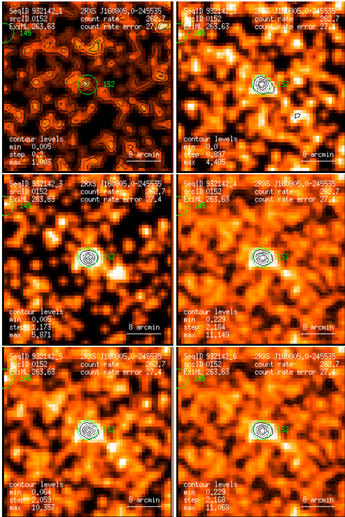
Figure 152: RASS 932142: detection 0152: band rate images, Gaussian filter: (1) PSPP channels 11 – 41, (2) 52 – 90, (3) 91 – 201, (4) 11 – 235, (5) 52 – 201, (6) 11 – 201. Broad band rates in counts/ks. Band rate contour levels in counts/ks/arcmin 2 .
