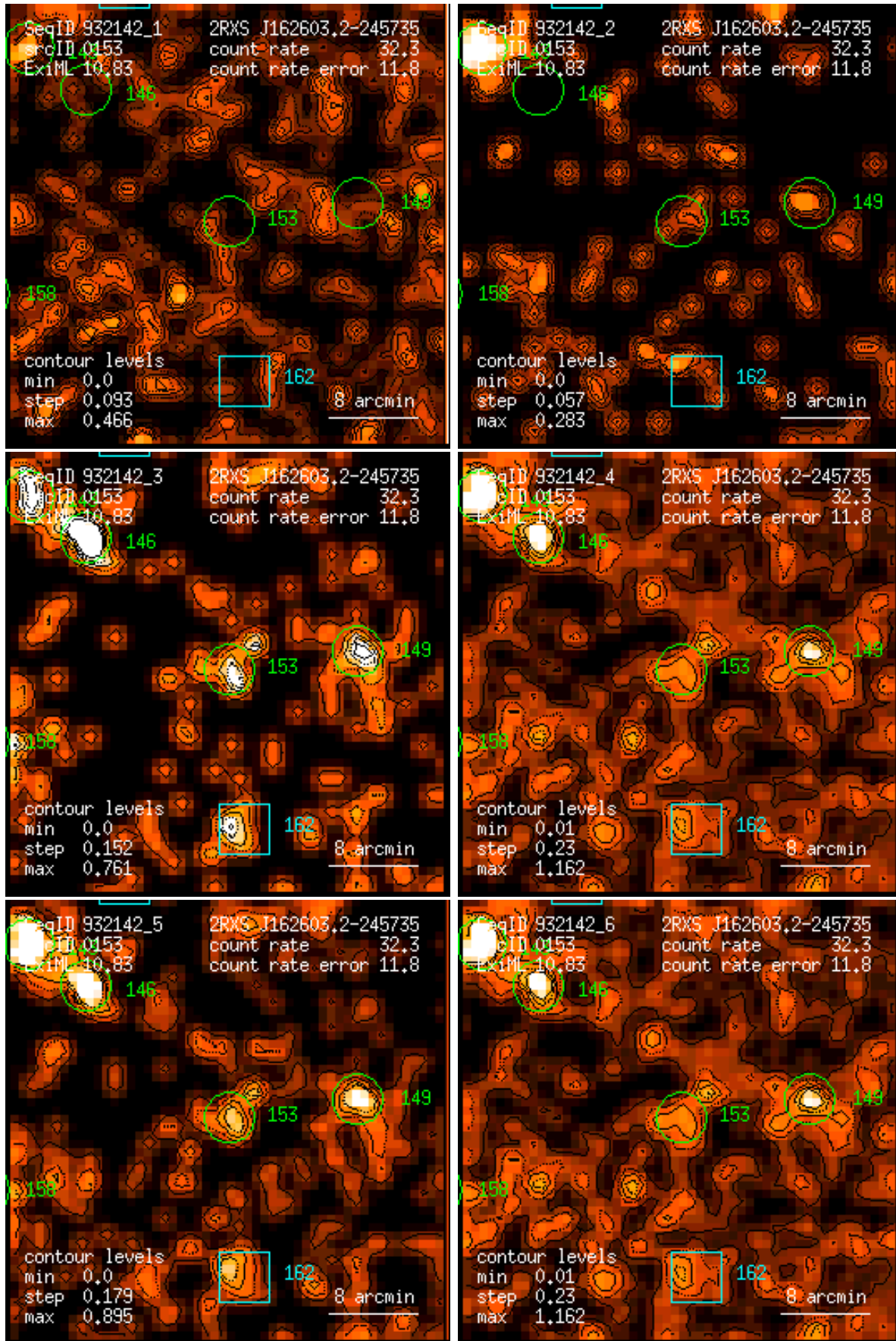
Figure 153: RASS 932142: detection 0153: band rate images, Gaussian filter: (1) PSPC channels 11 – 41, (2) 52 – 90, (3) 91 – 201, (4) 11 – 235, (5) 52 – 201, (6) 11 – 201. Broad band rates in counts/ks. Band rate contour levels in counts/ks/arcmin 2 .
