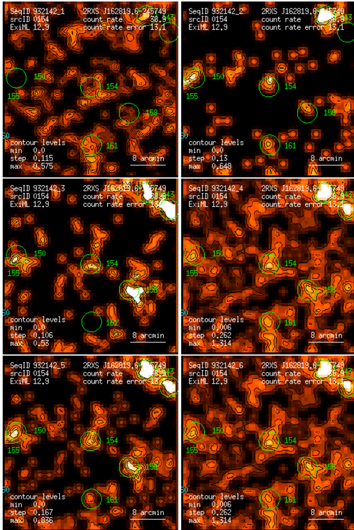
Figure 154: RASS 932142: detection 0154: band rate images, Gaussian filter: (1) PSPC channels 11 – 41, (2) 52 – 90, (3) 91 – 201, (4) 11 – 235, (5) 52 – 201, (6) 11 – 201. Broad band rates in counts/ks. Band rate contour levels in counts/ks/arcmin 2 .
