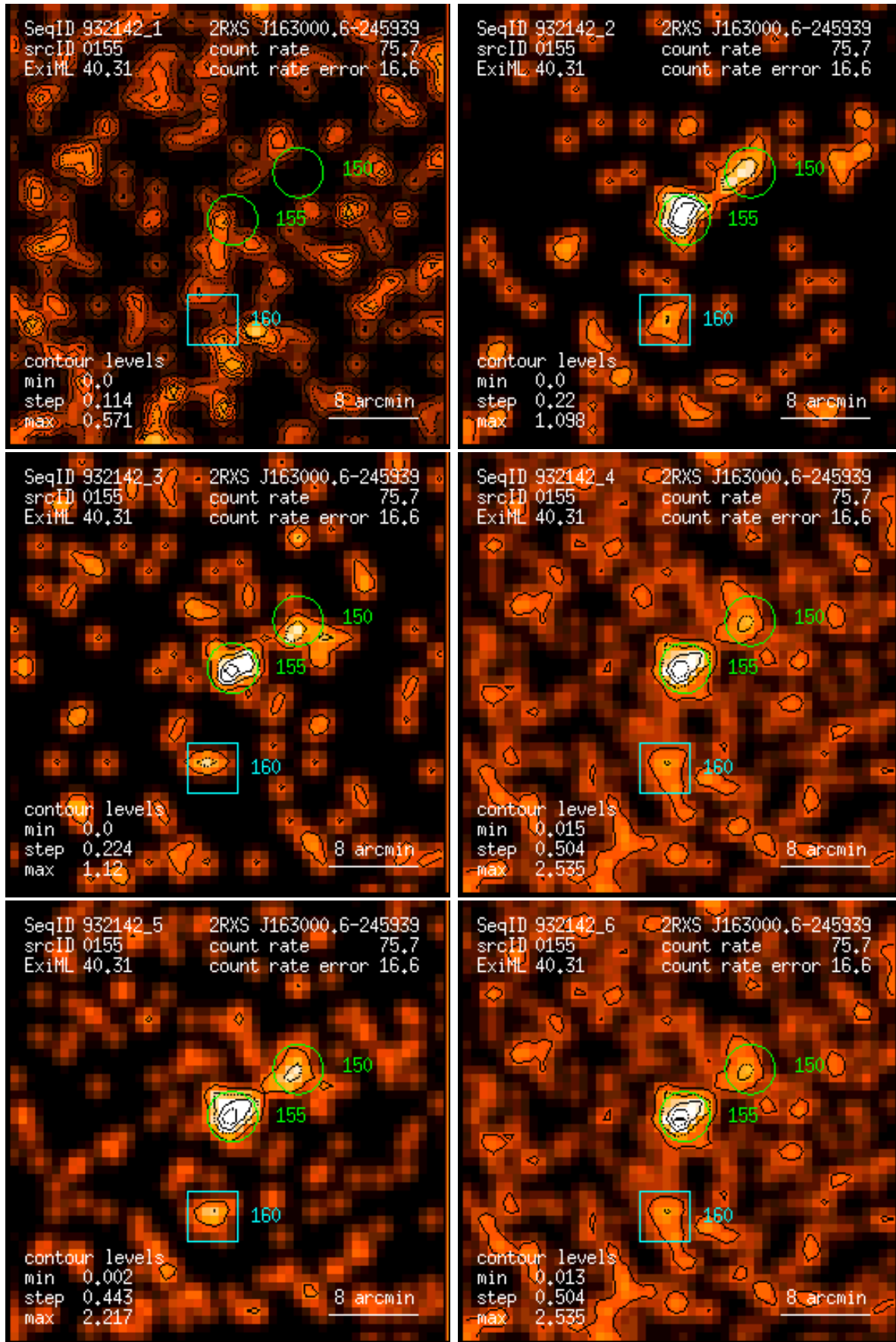
Figure 155: RASS 932142: detection 0155: band rate images, Gaussian filter: (1) PSPC channels 11 – 41, (2) 52 – 90, (3) 91 – 201, (4) 11 – 235, (5) 52 – 201, (6) 11 – 201. Broad band rates in counts/ks. Band rate contour levels in counts/ks/arcmin 2 .
