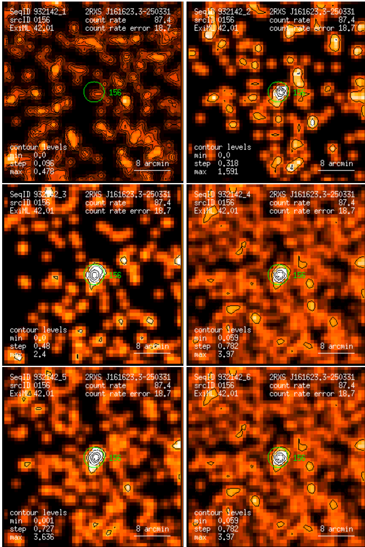
Figure 156: RASS 932142: detection 0156: band rate images, Gaussian filter: (1) PSPC channels 11 – 41, (2) 52 – 90, (3) 91 – 201, (4) 11 – 235, (5) 52 – 201, (6) 11 – 201. Broad band rates in counts/ks. Band rate contour levels in counts/ks/arcmin 2 .
