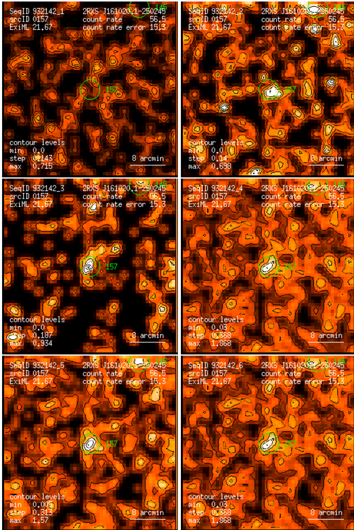
Figure 157: RASS 932142: detection 0157: band rate images, Gaussian filter: (1) PSPC channels 11 – 41, (2) 52 – 90, (3) 91 – 201, (4) 11 – 235, (5) 52 – 201, (6) 11 – 201. Broad band rates in counts/ks. Band rate contour levels in counts/ks/arcmin 2 .
