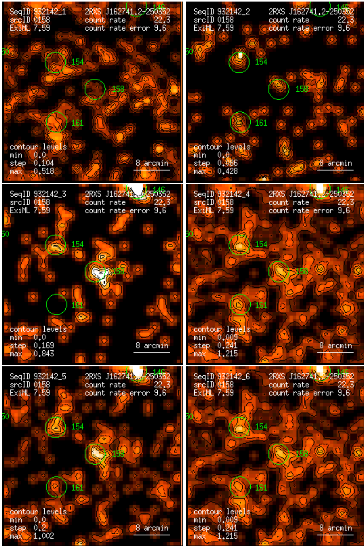
Figure 158: RASS 932142: detection 0158: band rate images, Gaussian filter: (1) PSPC channels 11 – 41, (2) 52 – 90, (3) 91 – 201, (4) 11 – 235, (5) 52 – 201, (6) 11 – 201. Broad band rates in counts/ks. Band rate contour levels in counts/ks/arcmin 2 .
