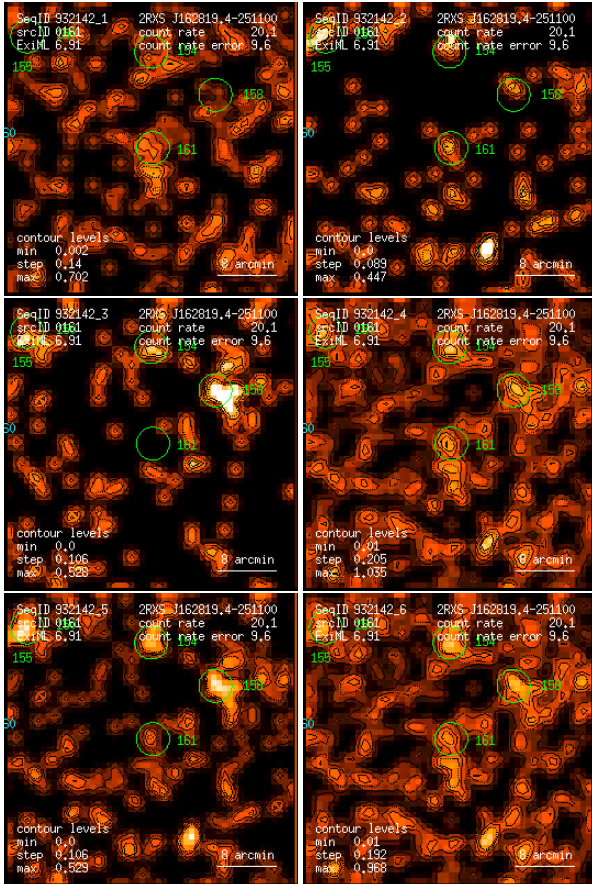
Figure 161: RASS 932142: detection 0161: band rate images, Gaussian filter: (1) PSPC channels 11 – 41, (2) 52 – 90, (3) 91 – 201, (4) 11 – 235, (5) 52 – 201, (6) 11 – 201. Broad band rates in counts/ks. Band rate contour levels in counts/ks/arcmin 2 .
