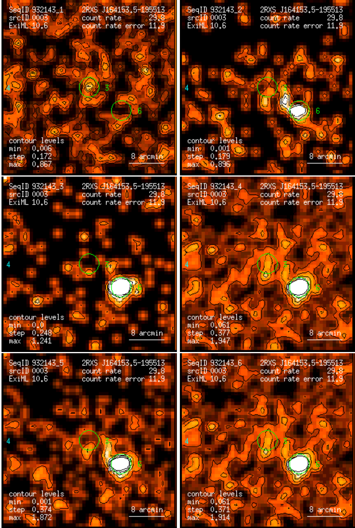
Figure 3: RASS 932143: detection 0003: band rate images, Gaussian filter: (1) PSPC channels 11 – 41, (2) 52 – 90, (3) 91 – 201, (4) 11 – 235, (5) 52 – 201, (6) 11 – 201. Broad band rates in counts/ks. Band rate contour levels in counts/ks/arcmin 2 .
