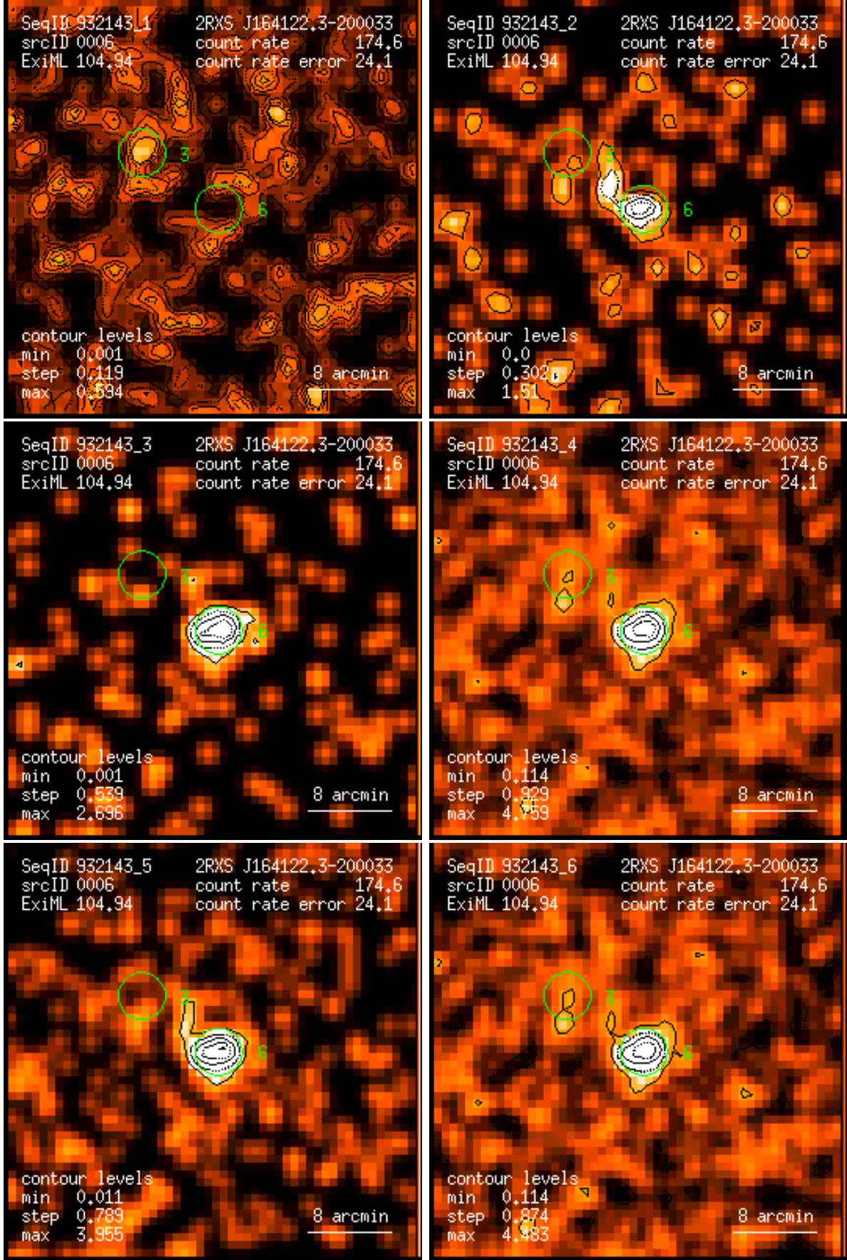
Figure 6: RASS 932143: detection 0006: band rate images, Gaussian filter: (1) PSPC channels 11 – 41, (2) 52 – 90, (3) 91 – 201, (4) 11 – 235, (5) 52 – 201, (6) 11 – 201. Broad band rates in counts/ks. Band rate contour levels in counts/ks/arcmin 2 .
