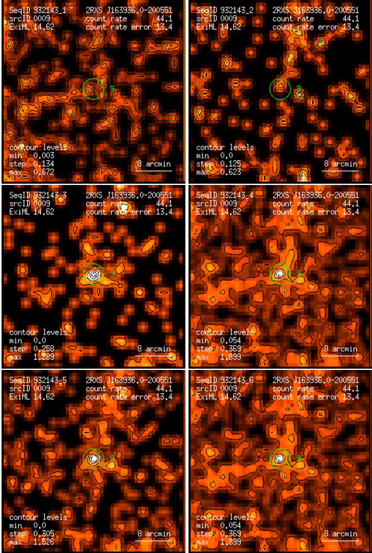
Figure 9: RASS 932143: detection 0009: band rate images, Gaussian filter: (1) PSPC channels 11 – 41, (2) 52 – 90, (3) 91 – 201, (4) 11 – 235, (5) 52 – 201, (6) 11 – 201. Broad band rates in counts/ks. Band rate contour levels in counts/ks/arcmin 2 .
