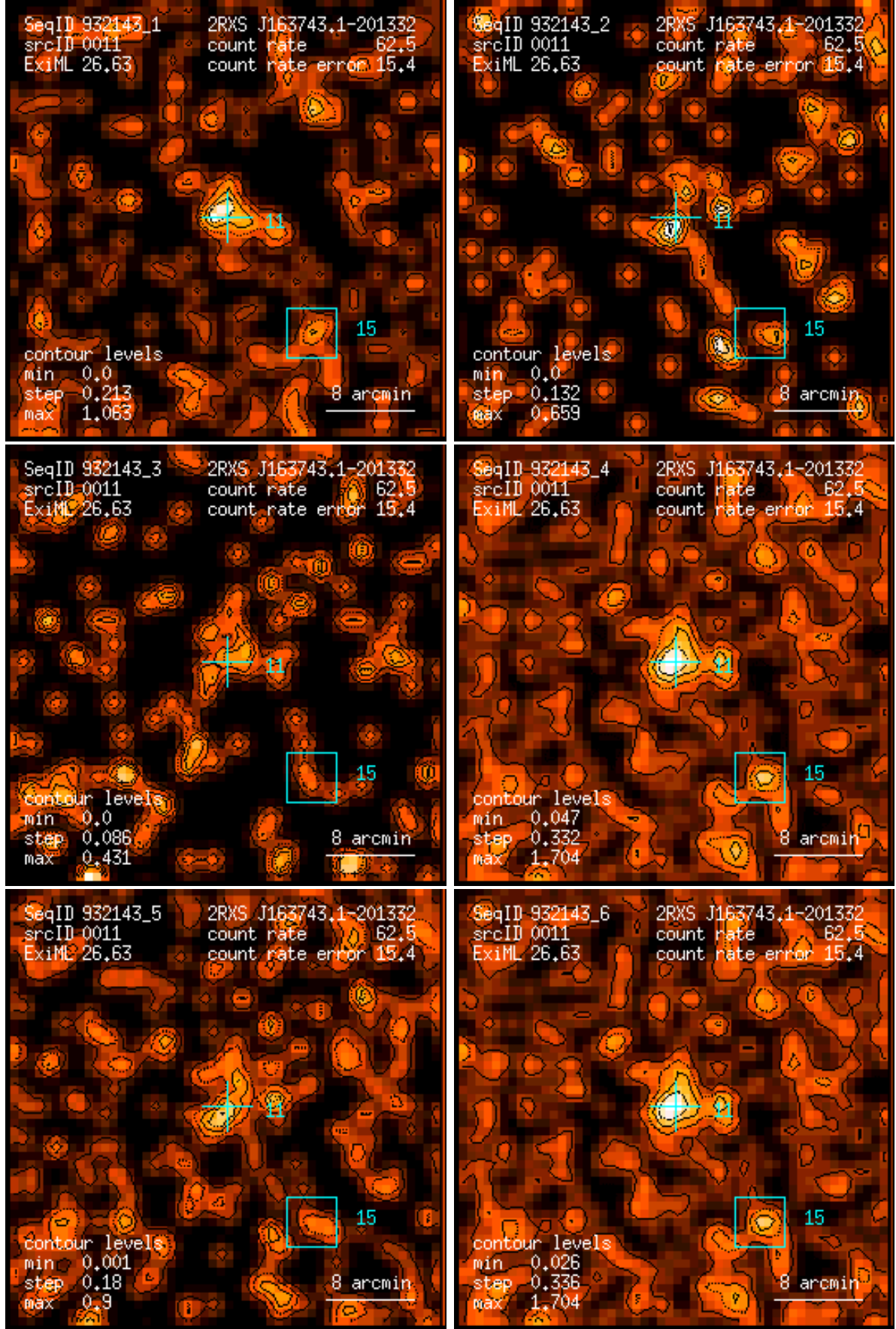
Figure 11: RASS 932143: detection 0011: band rate images, Gaussian filter: (1) PSPC channels 11 – 41, (2) 52 – 90, (3) 91 – 201, (4) 11 – 235, (5) 52 – 201, (6) 11 – 201. Broad band rates in counts/ks. Band rate contour levels in counts/ks/arcmin 2 .
