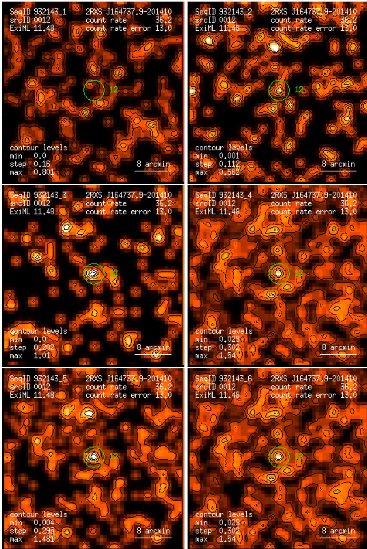
Figure 12: RASS 932143: detection 0012: band rate images, Gaussian filter: (1) PSPC channels 11 – 41, (2) 52 – 90, (3) 91 – 201, (4) 11 – 235, (5) 52 – 201, (6) 11 – 201. Broad band rates in counts/ks. Band rate contour levels in counts/ks/arcmin 2 .
