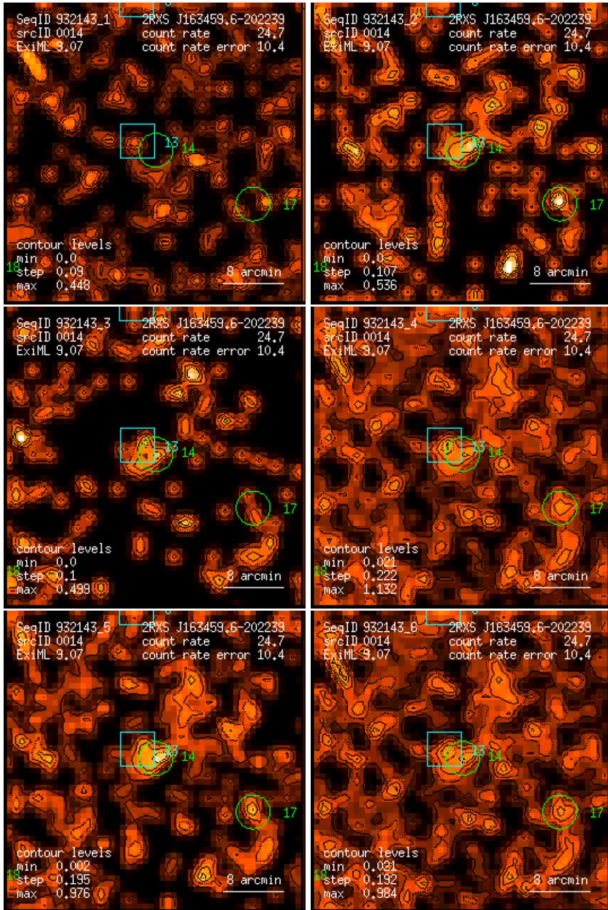
Figure 14: RASS 932143: detection 0014: band rate images, Gaussian filter: (1) PSPC channels 11 – 41, (2) 52 – 90, (3) 91 – 201, (4) 11 – 235, (5) 52 – 201, (6) 11 – 201. Broad band rates in counts/ks. Band rate contour levels in counts/ks/arcmin 2 .
