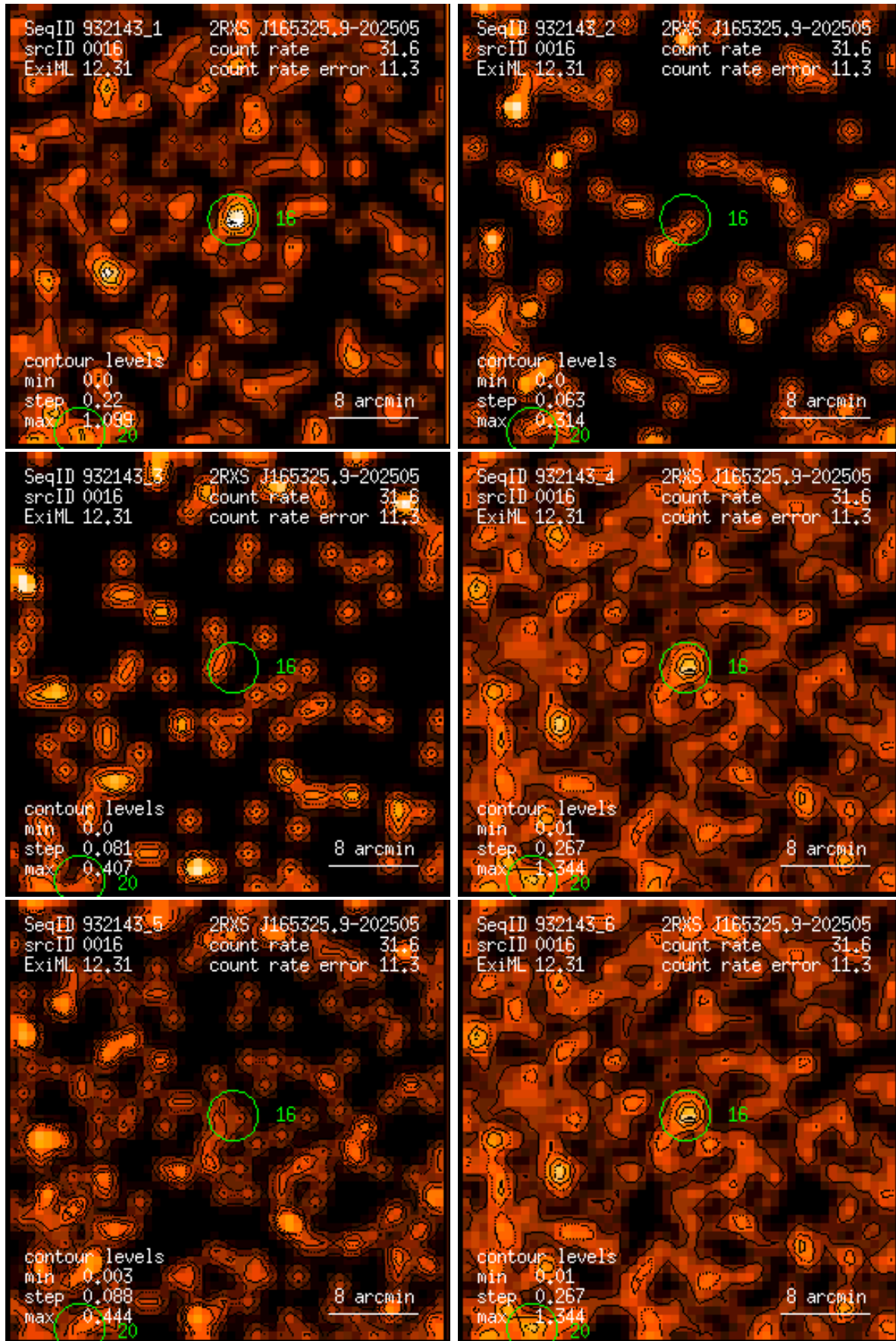
Figure 16: RASS 932143: detection 0016: band rate images, Gaussian filter: (1) PSPC channels 11 – 41, (2) 52 – 90, (3) 91 – 201, (4) 11 – 235, (5) 52 – 201, (6) 11 – 201. Broad band rates in counts/ks. Band rate contour levels in counts/ks/arcmin 2 .
