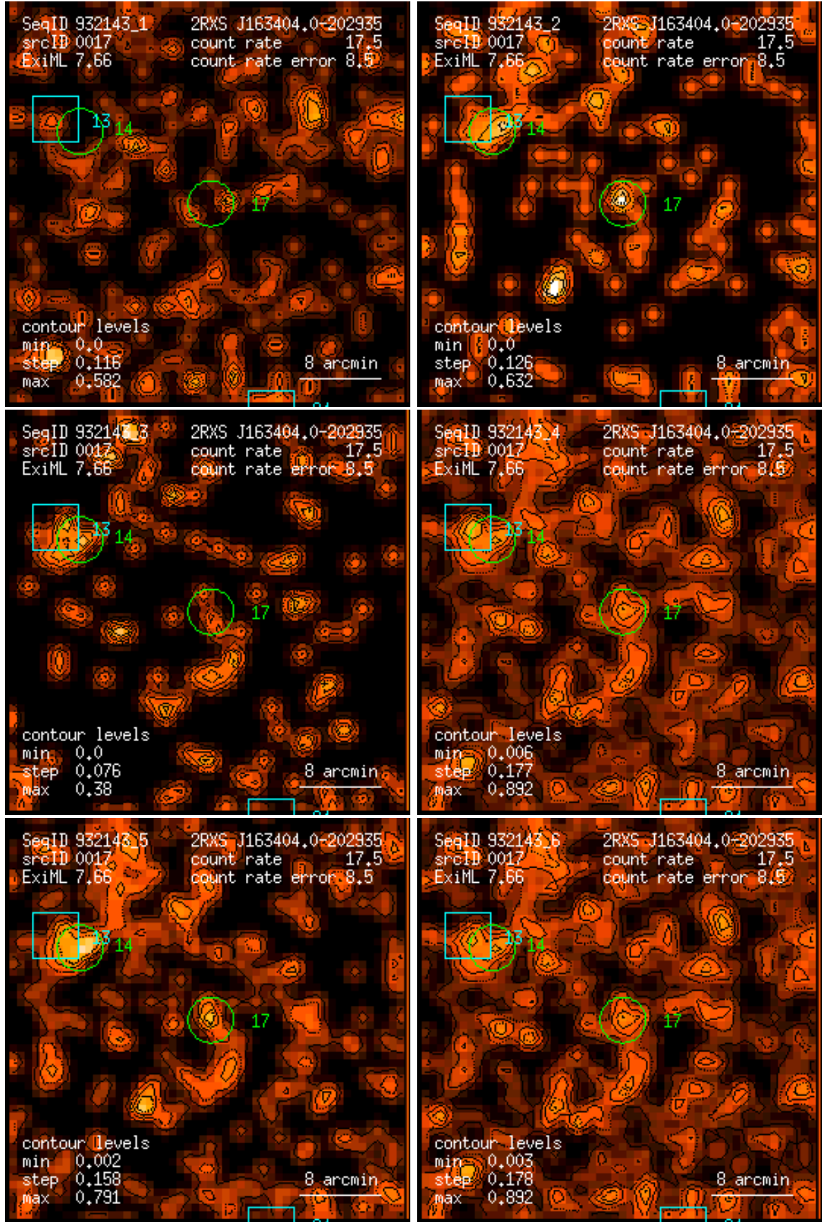
Figure 17: RASS 932143: detection 0017: band rate images, Gaussian filter: (1) PSPC channels 11 – 41, (2) 52 – 90, (3) 91 – 201, (4) 11 – 235, (5) 52 – 201, (6) 11 – 201. Broad band rates in counts/ks. Band rate contour levels in counts/ks/arcmin 2 .
