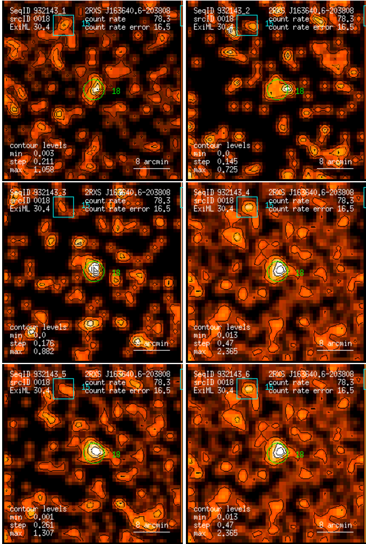
Figure 18: RASS 932143: detection 0018: band rate images, Gaussian filter: (1) PSPC channels 11 – 41, (2) 52 – 90, (3) 91 – 201, (4) 11 – 235, (5) 52 – 201, (6) 11 – 201. Broad band rates in counts/ks. Band rate contour levels in counts/ks/arcmin 2 .
