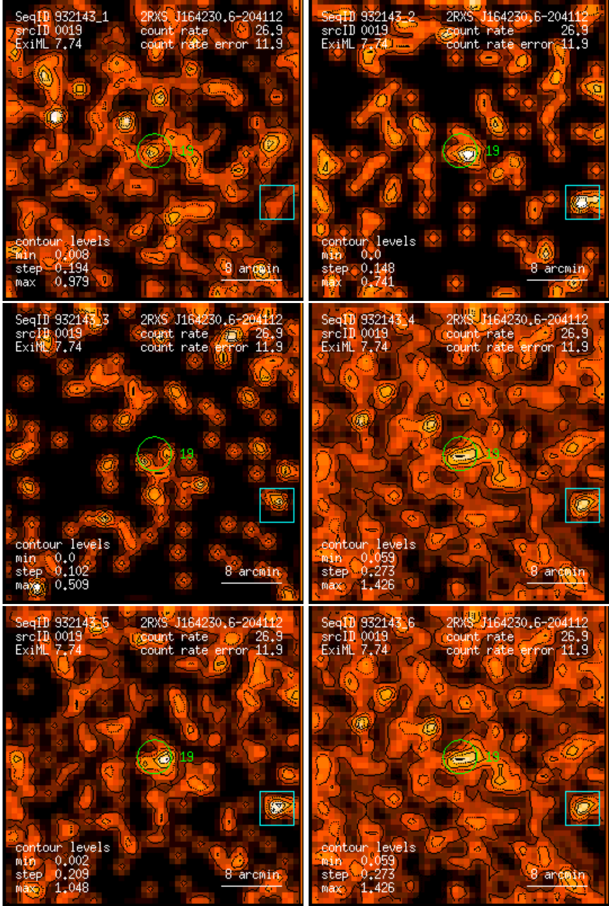
Figure 19: RASS 932143: detection 0019: band rate images, Gaussian filter: (1) PSPC channels 11 – 41, (2) 52 – 90, (3) 91 – 201, (4) 11 – 235, (5) 52 – 201, (6) 11 – 201. Broad band rates in counts/ks. Band rate contour levels in counts/ks/arcmin 2 .
