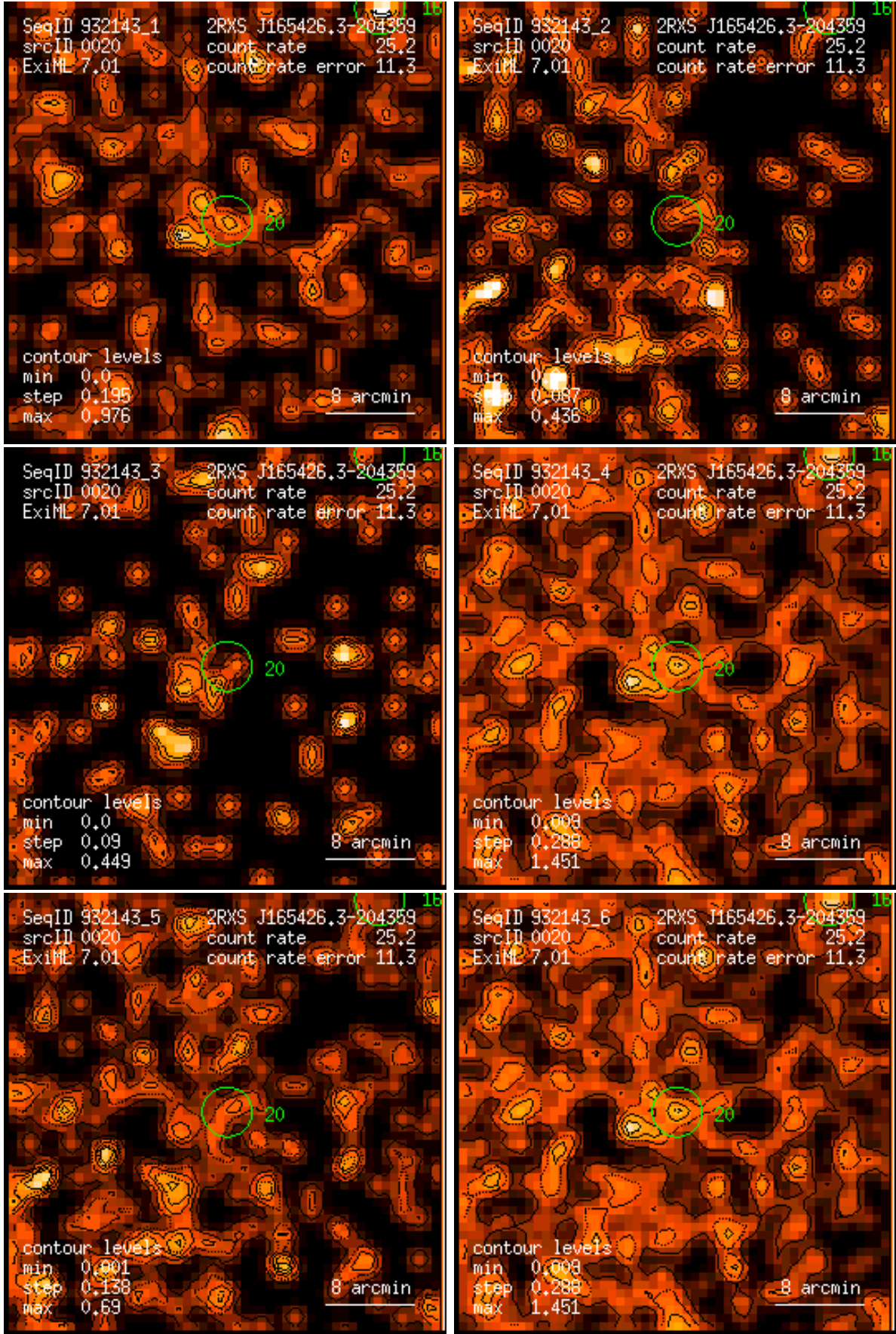
Figure 20: RASS 932143: detection 0020: band rate images, Gaussian filter: (1) PSPC channels 11 – 41, (2) 52 – 90, (3) 91 – 201, (4) 11 – 235, (5) 52 – 201, (6) 11 – 201. Broad band rates in counts/ks. Band rate contour levels in counts/ks/arcmin 2 .
