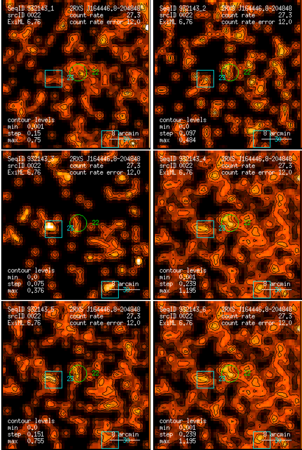
Figure 22: RASS 932143: detection 0022: band rate images, Gaussian filter: (1) PSPC channels 11 – 41, (2) 52 – 90, (3) 91 – 201, (4) 11 – 235, (5) 52 – 201, (6) 11 – 201. Broad band rates in counts/ks. Band rate contour levels in counts/ks/arcmin 2 .
