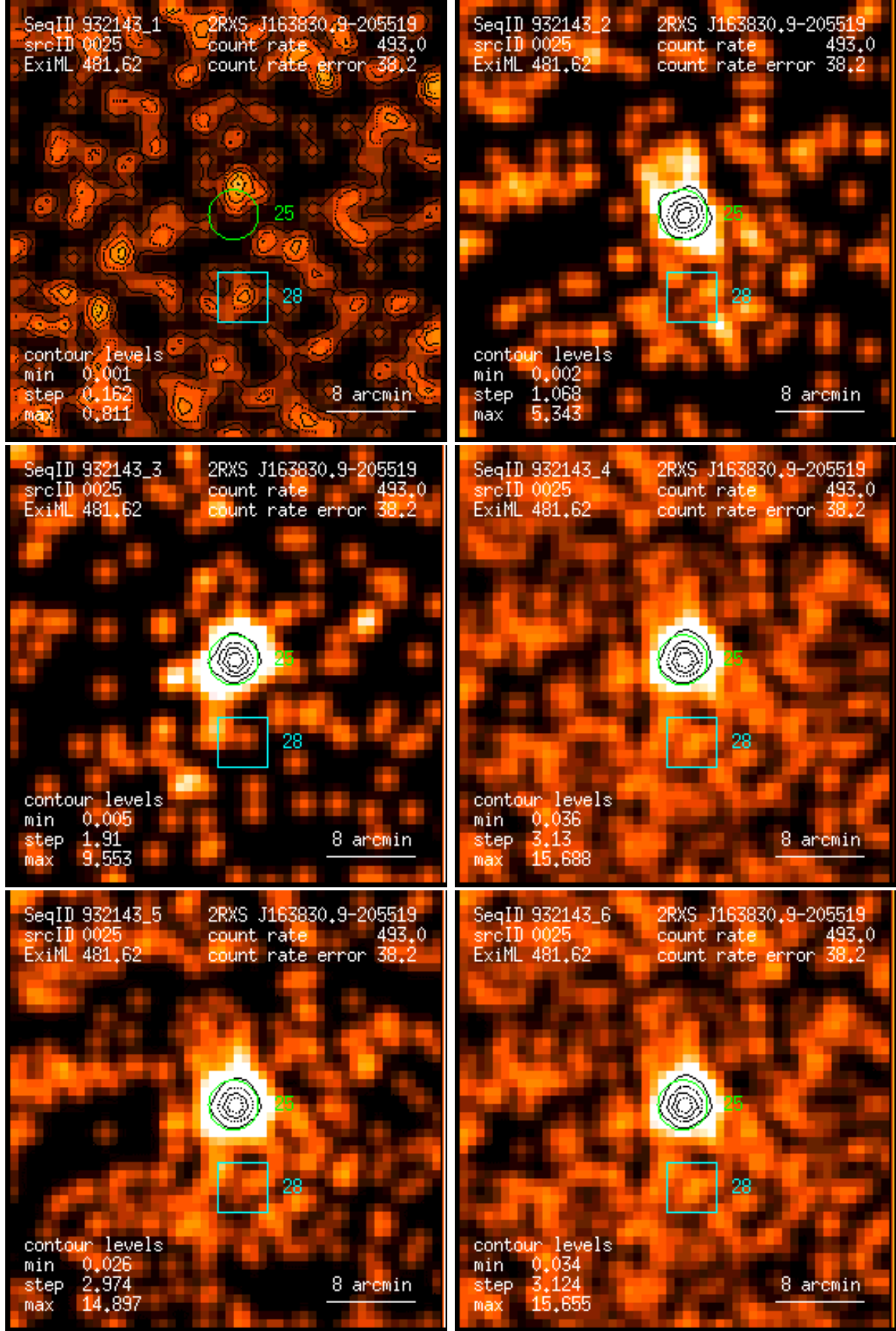
Figure 25: RASS 932143: detection 0025: band rate images, Gaussian filter: (1) PSPC channels 11 – 41, (2) 52 – 90, (3) 91 – 201, (4) 11 – 235, (5) 52 – 201, (6) 11 – 201. Broad band rates in counts/ks. Band rate contour levels in counts/ks/arcmin 2 .
