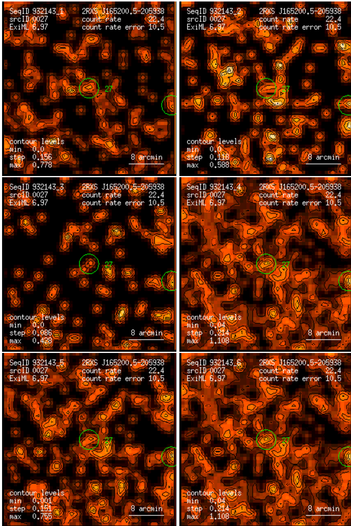
Figure 27: RASS 932143: detection 0027: band rate images, Gaussian filter: (1) PSPC channels 11 – 41, (2) 52 – 90, (3) 91 – 201, (4) 11 – 235, (5) 52 – 201, (6) 11 – 201. Broad band rates in counts/ks. Band rate contour levels in counts/ks/arcmin 2 .
