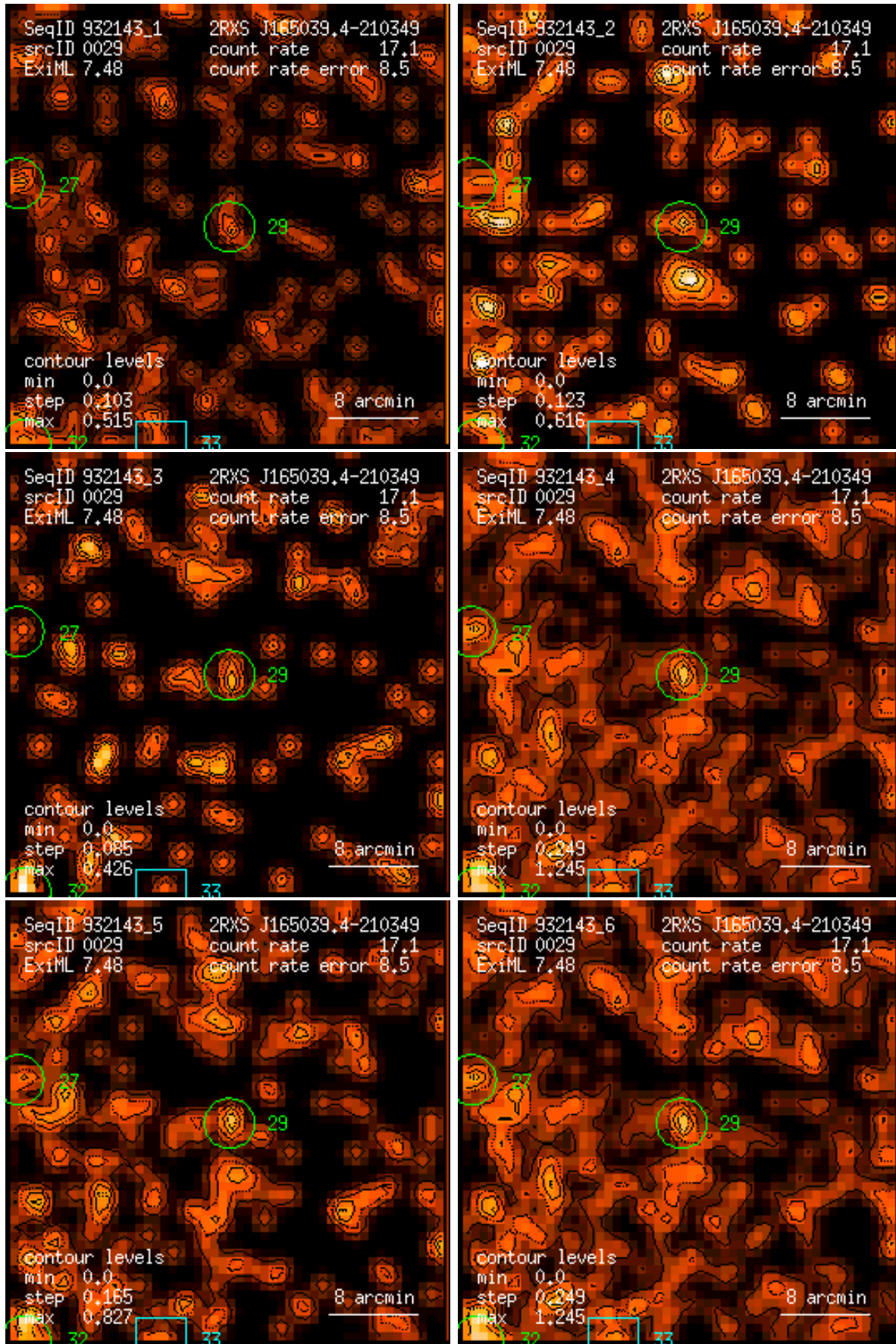
Figure 29: RASS 932143: detection 0029: band rate images, Gaussian filter: (1) PSPC channels 11 – 41, (2) 52 – 90, (3) 91 – 201, (4) 11 – 235, (5) 52 – 201, (6) 11 – 201. Broad band rates in counts/ks. Band rate contour levels in counts/ks/arcmin 2 .
